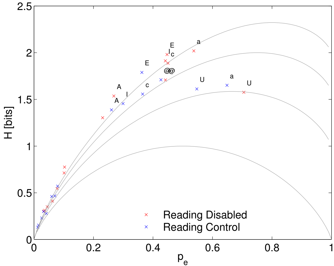
H(p e ) for Targets (vowels) in Final Position
