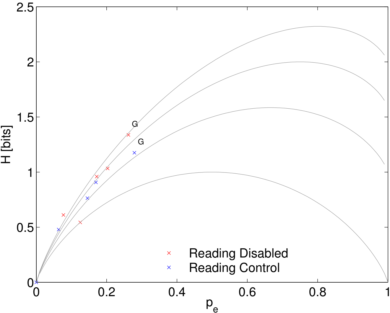
H(p_e) for Targets (nasalsLiquidsGlides) in Final Position
