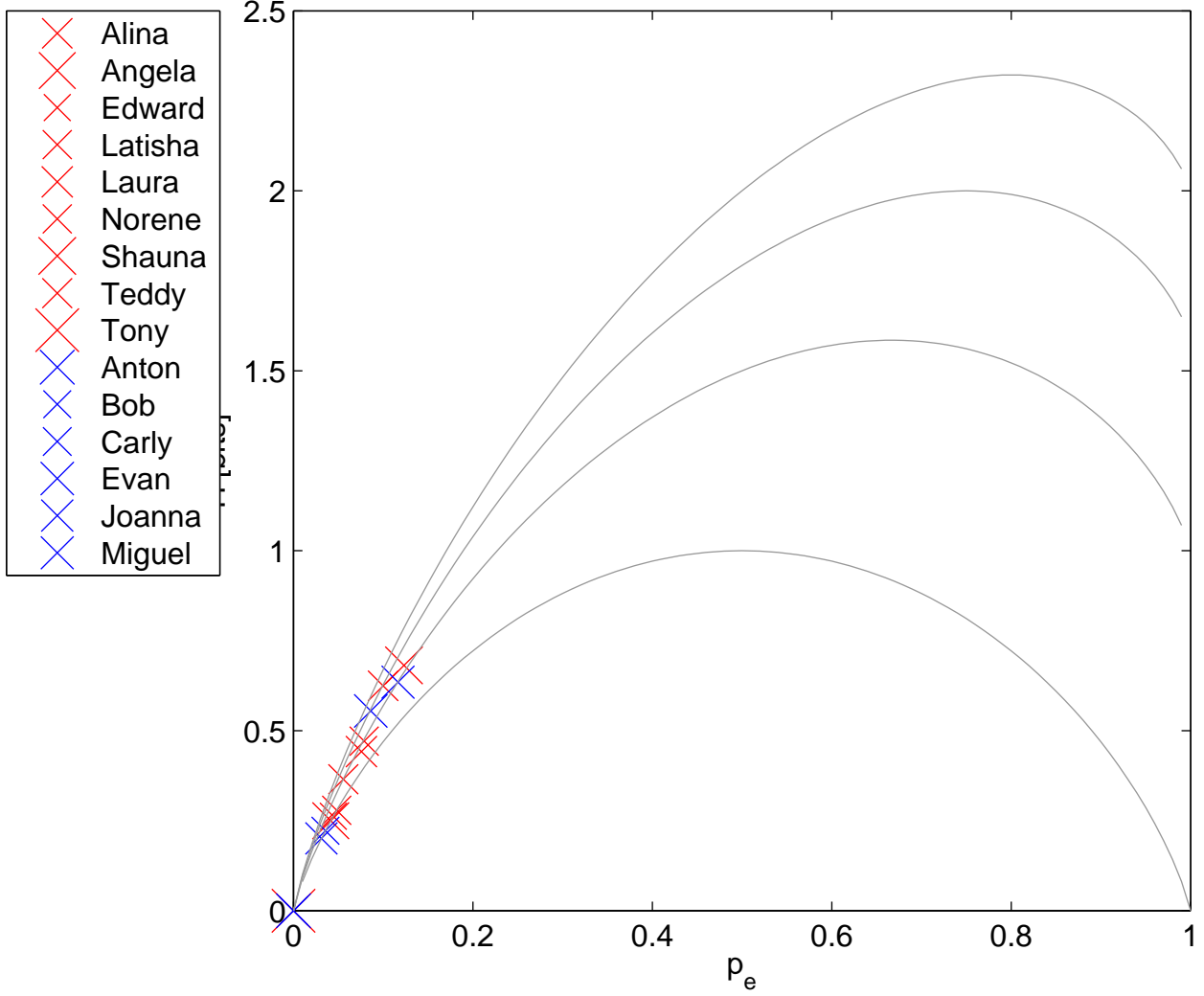
H(p e ) for Letter (k) in Final Position
