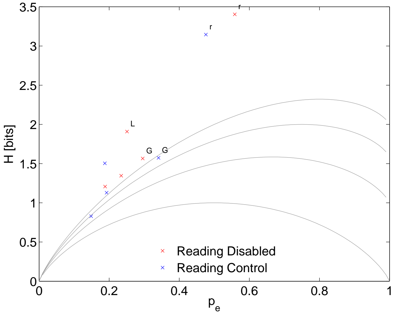
H(p_e) for Targets (nasalsLiquidsGlides) in Final Position
