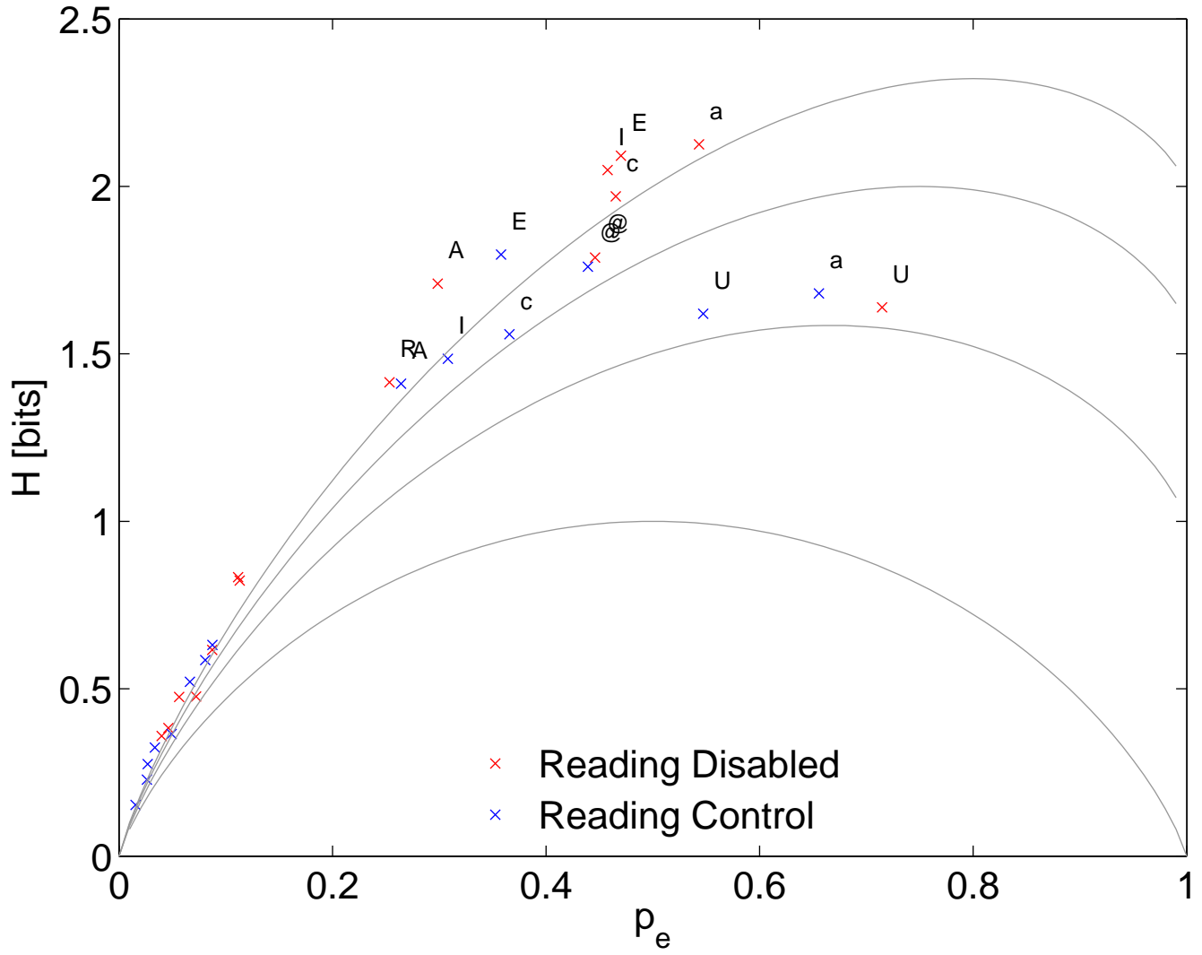
H(p_e) for Targets (vowels) in Final Position
