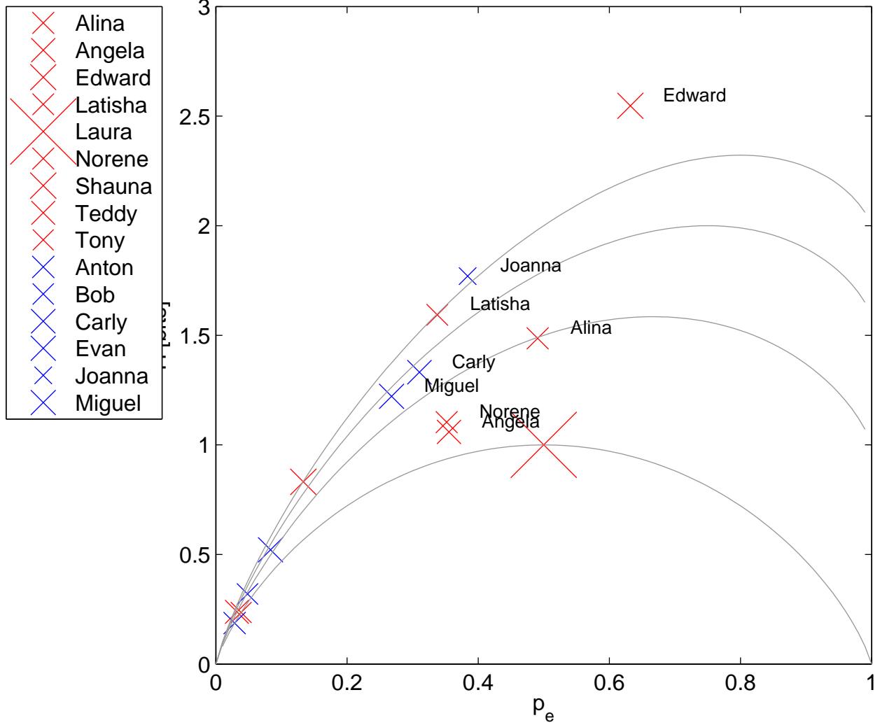
H(p_e) for Letter (z) in Final Position
