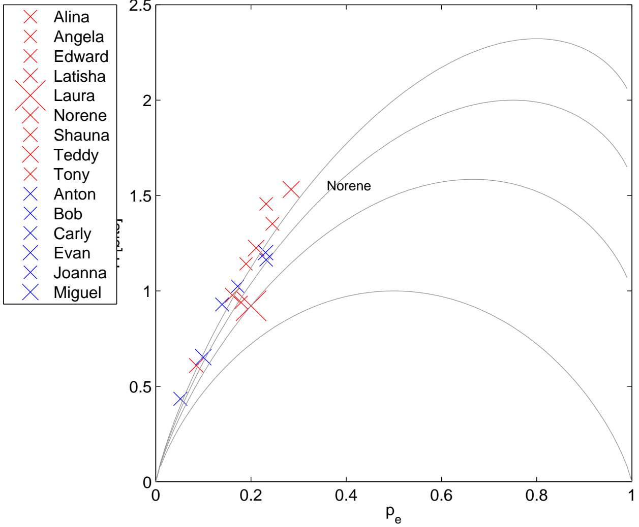
H(p e ) for Letter (e) in Initial Position
