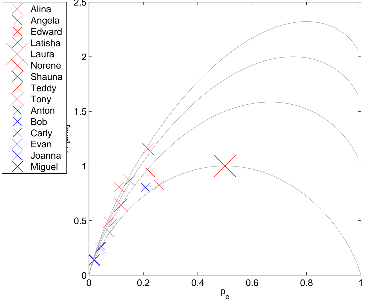
H(p e ) for Letter (J) in Initial Position
