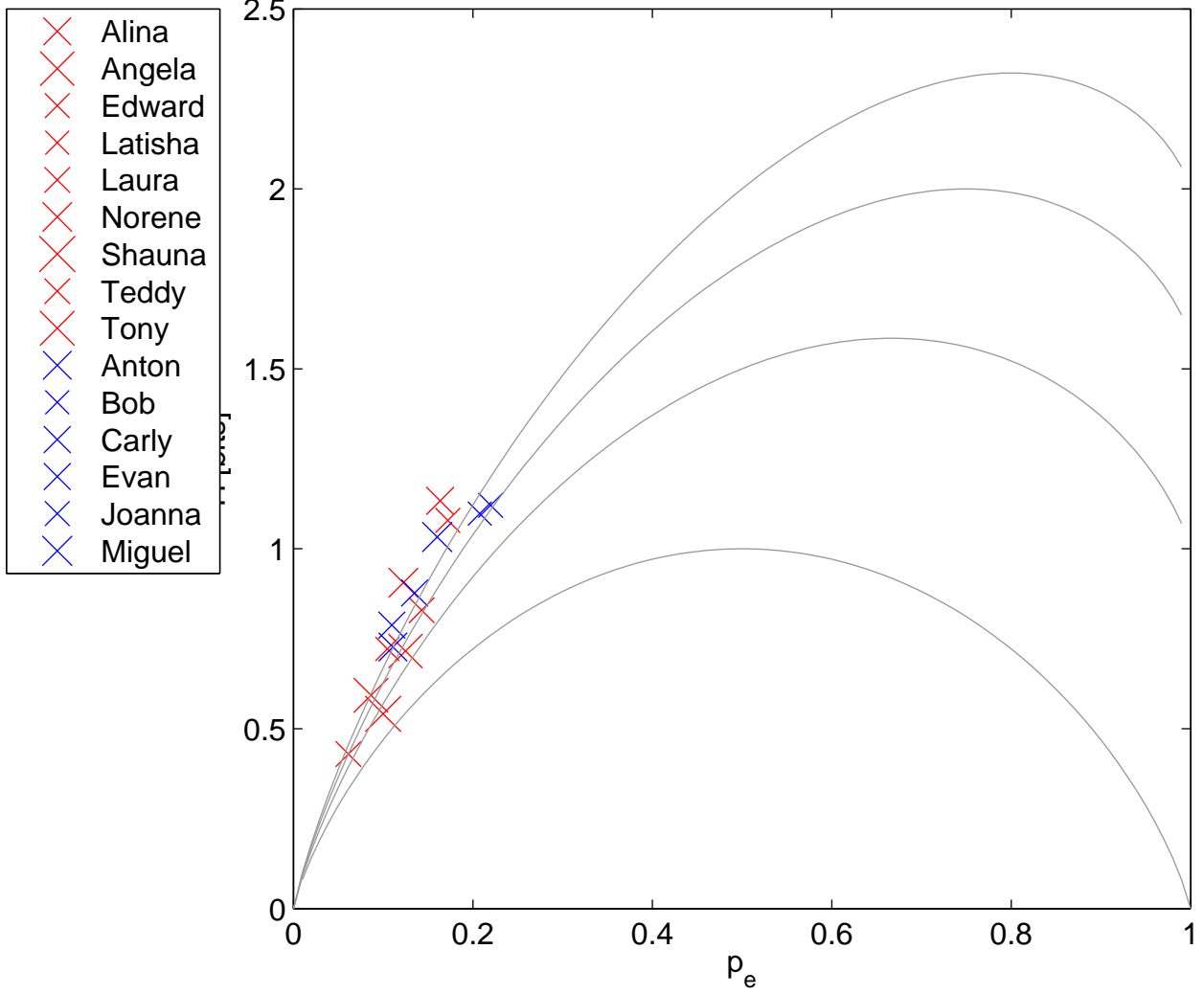
H(p e ) for Letter (u) in Initial Position
