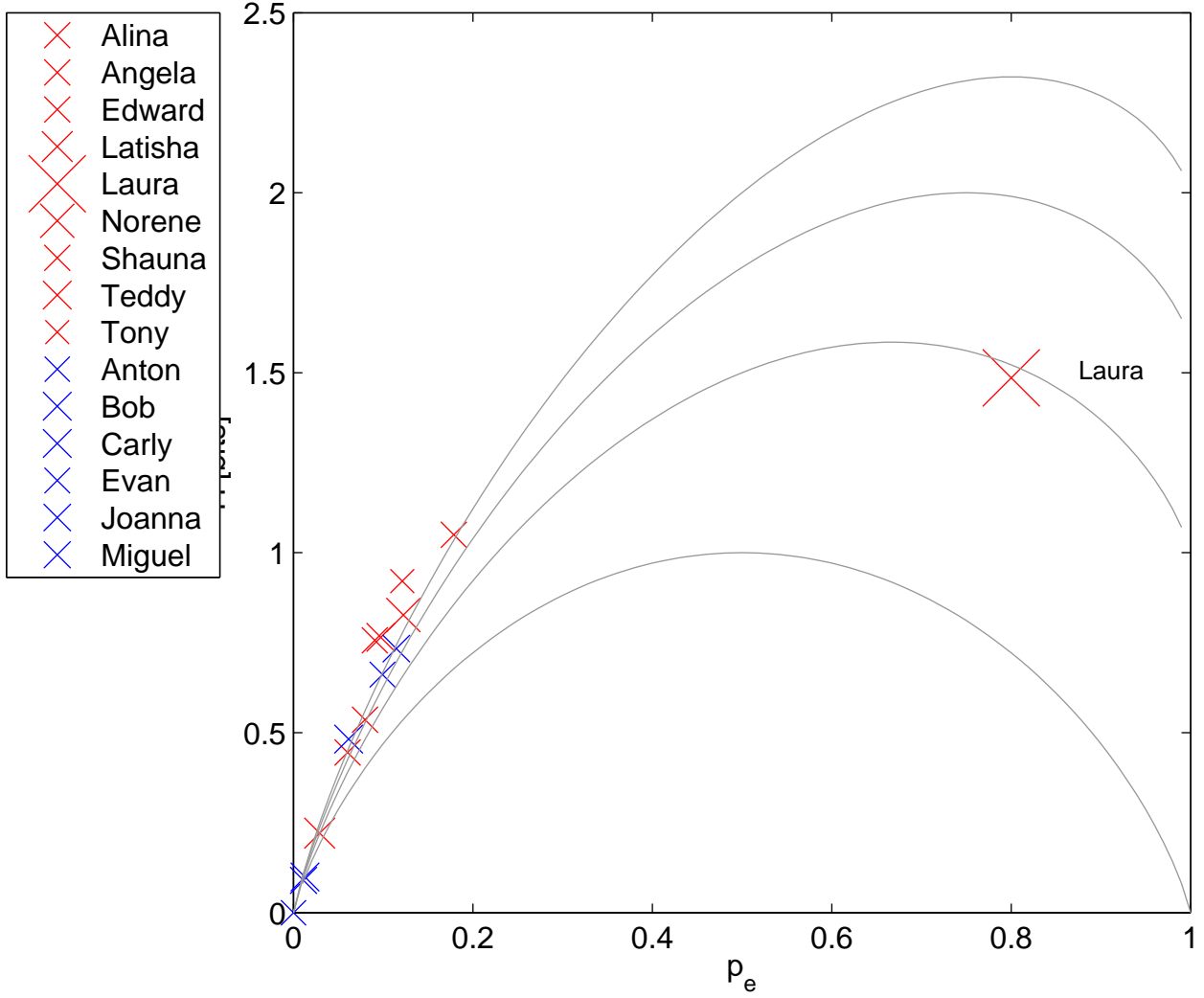
H(p e ) for Letter (Y) in Initial Position
