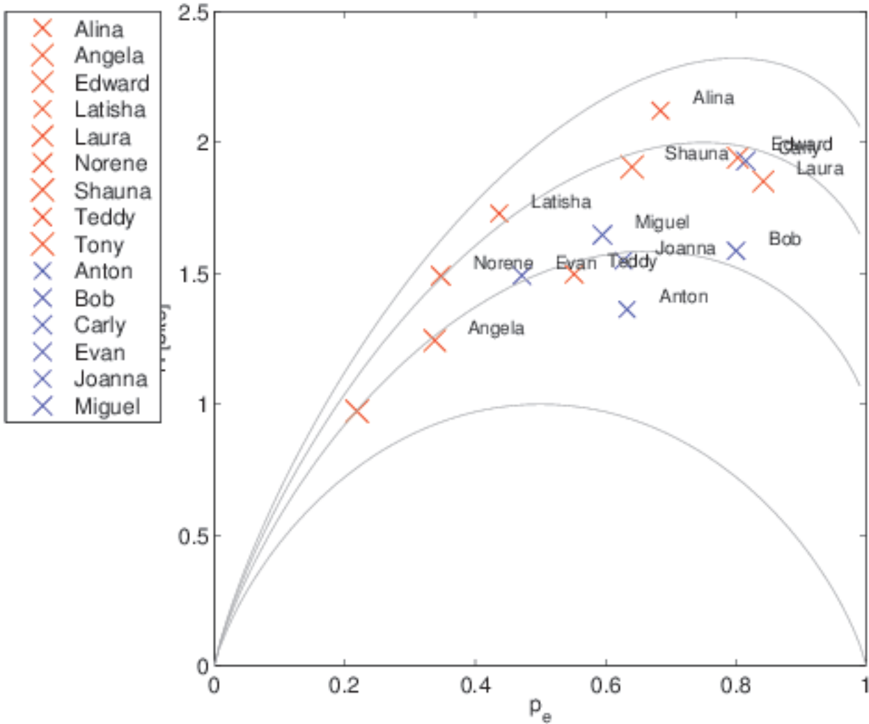
H(p_e) for Letter (a) in Final Position
