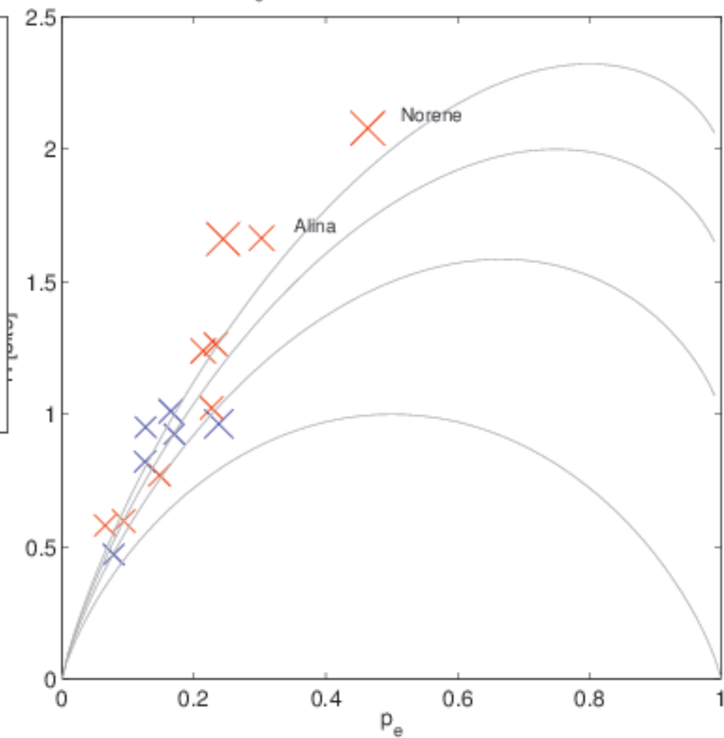
H(p_e) for Letter (b) in Final Position
