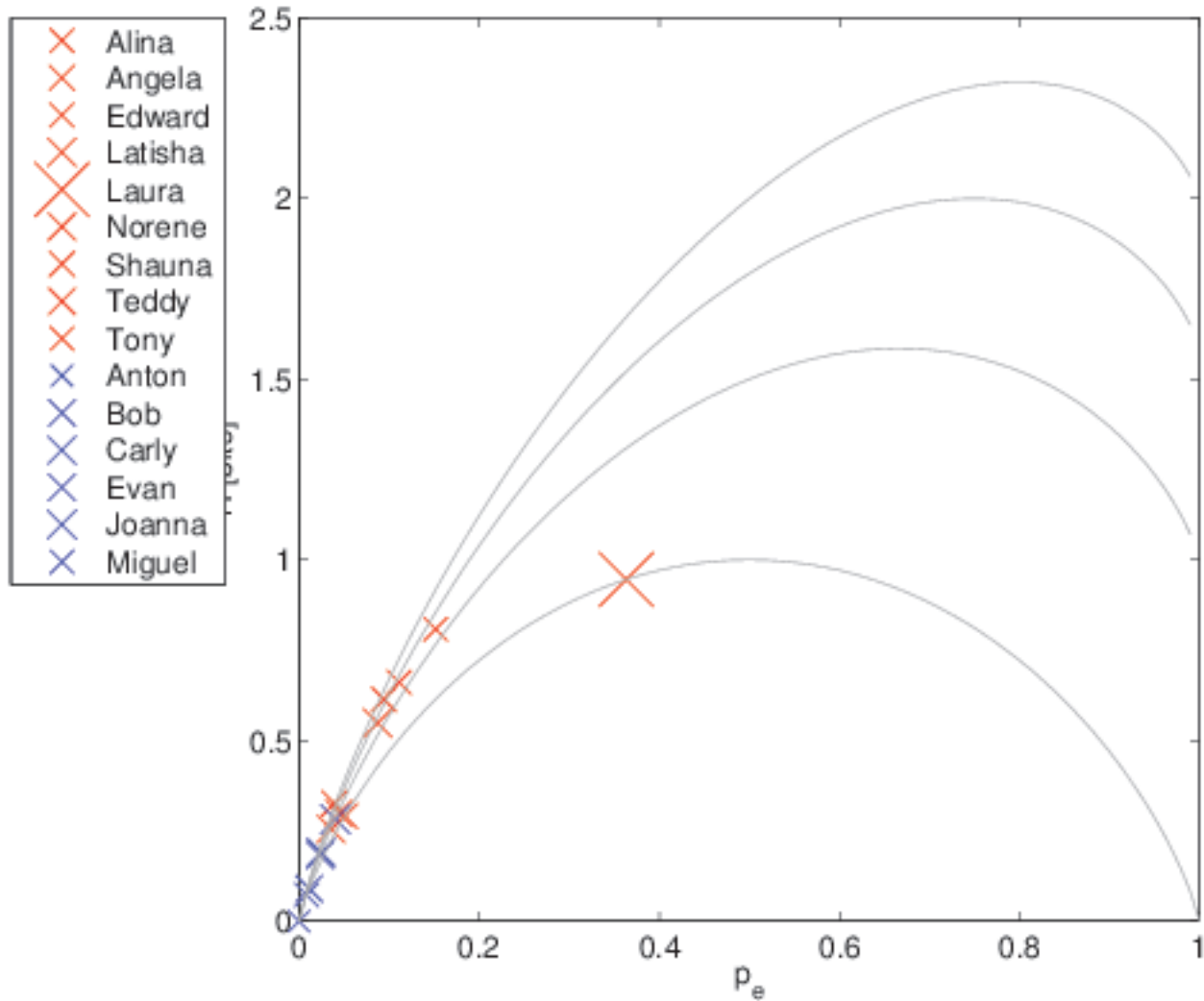
H(p_e) for Letter (e) in Final Position
