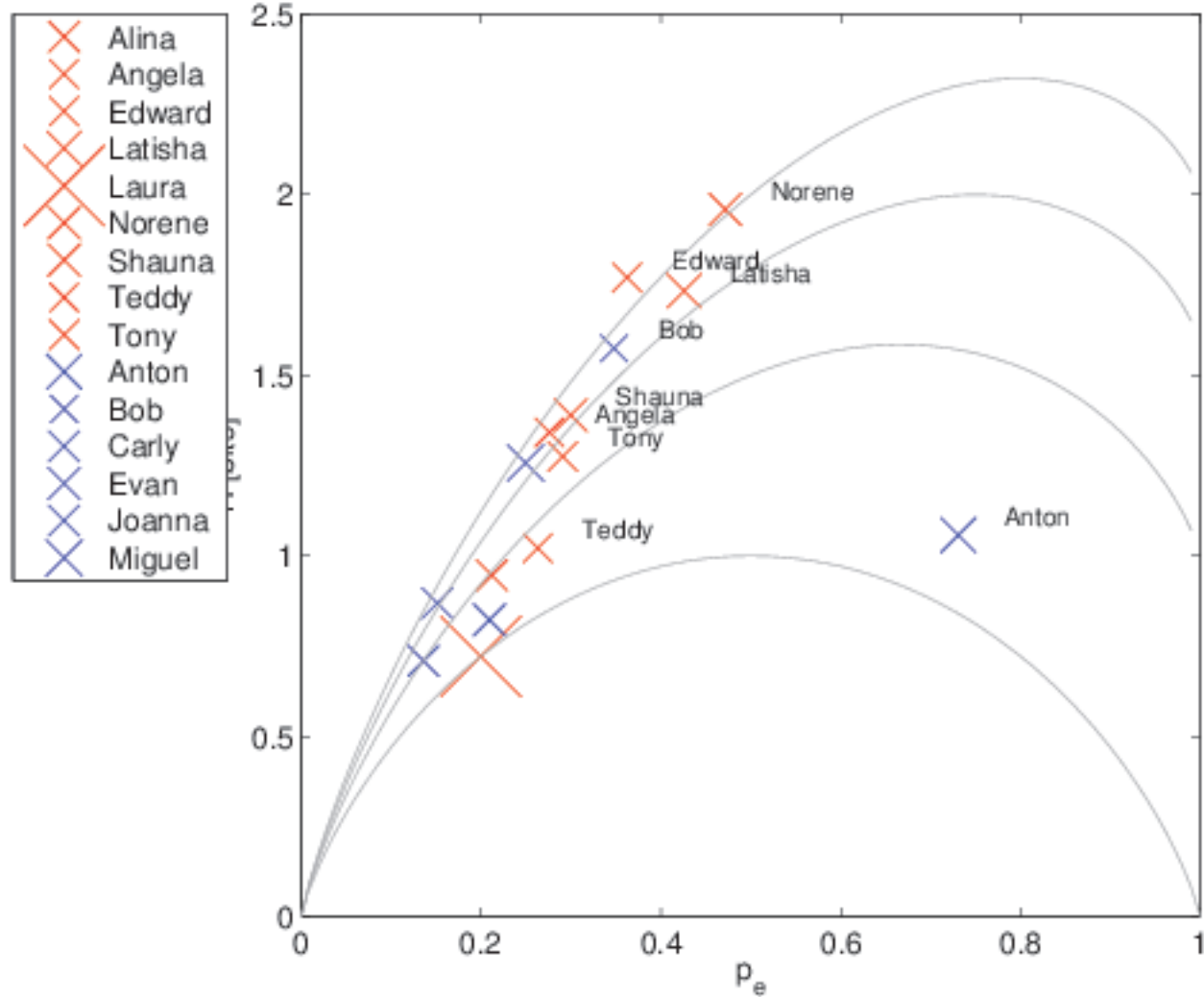
H(p_e) for Letter (f) in Final Position
