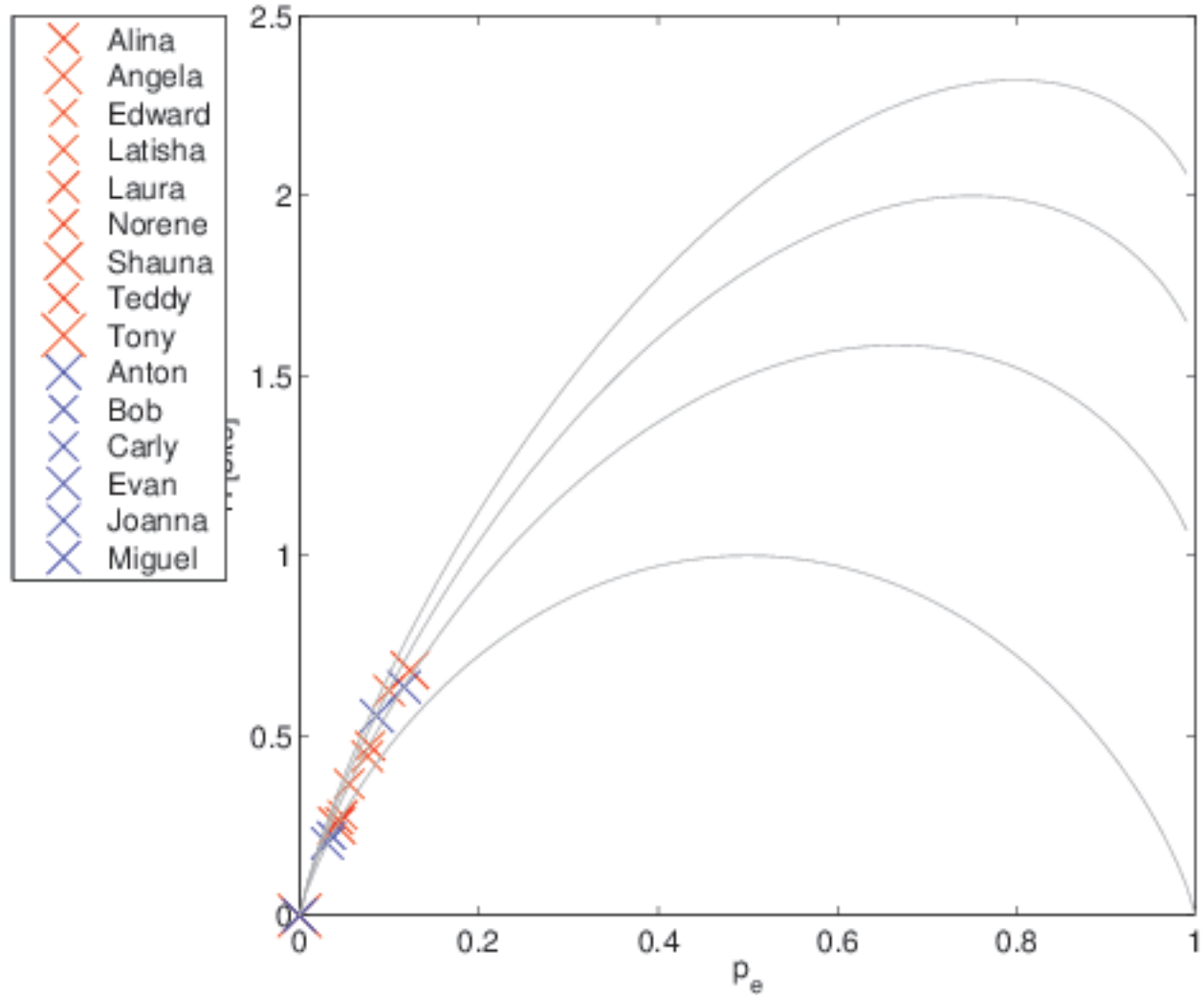
H(p_e) for Letter (k) in Final Position
