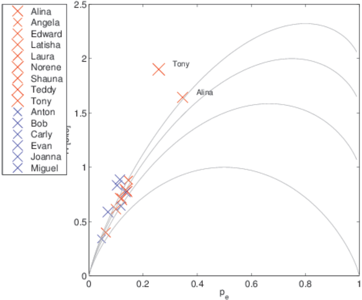
H(p_e) for Letter (p) in Final Position
