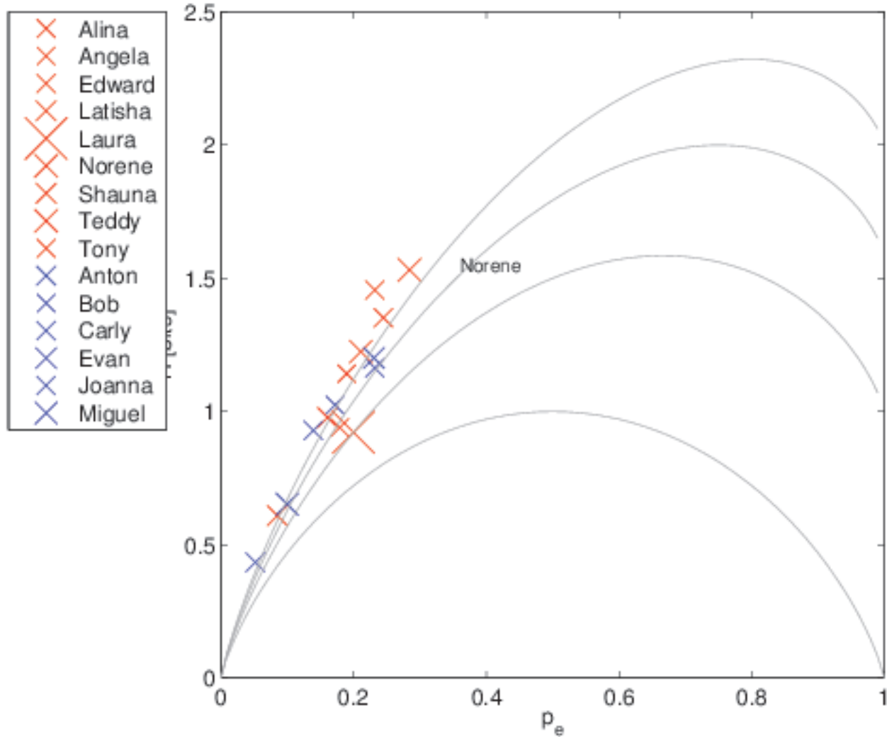
H(p_e) for Letter (e) in Initial Position
