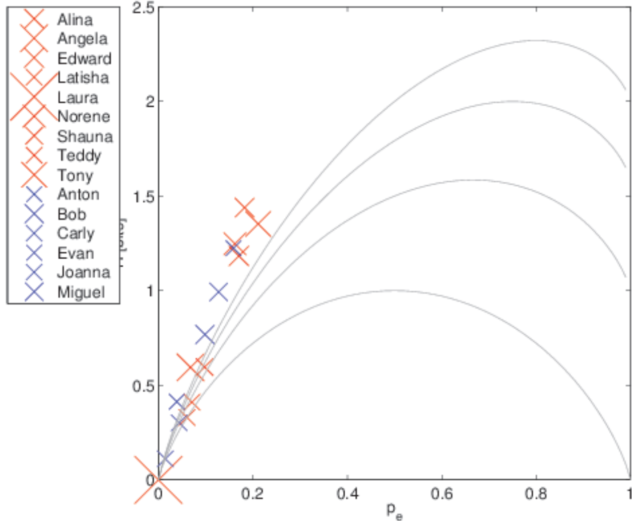
H(p_e) for Letter (h) in Initial Position
