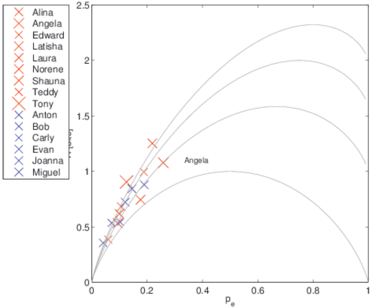
H(p_e) for Letter (i) in Initial Position
