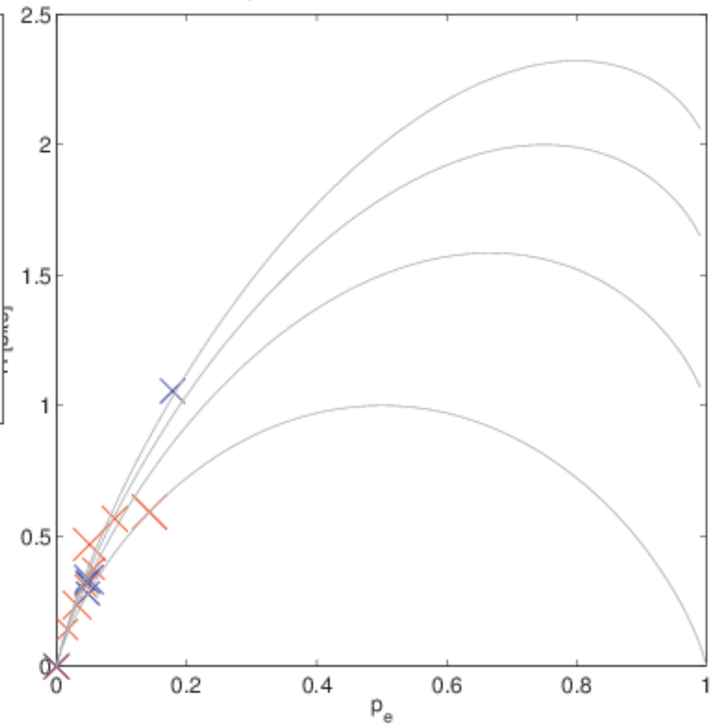
H(p_e) for Letter (k) in Initial Position
