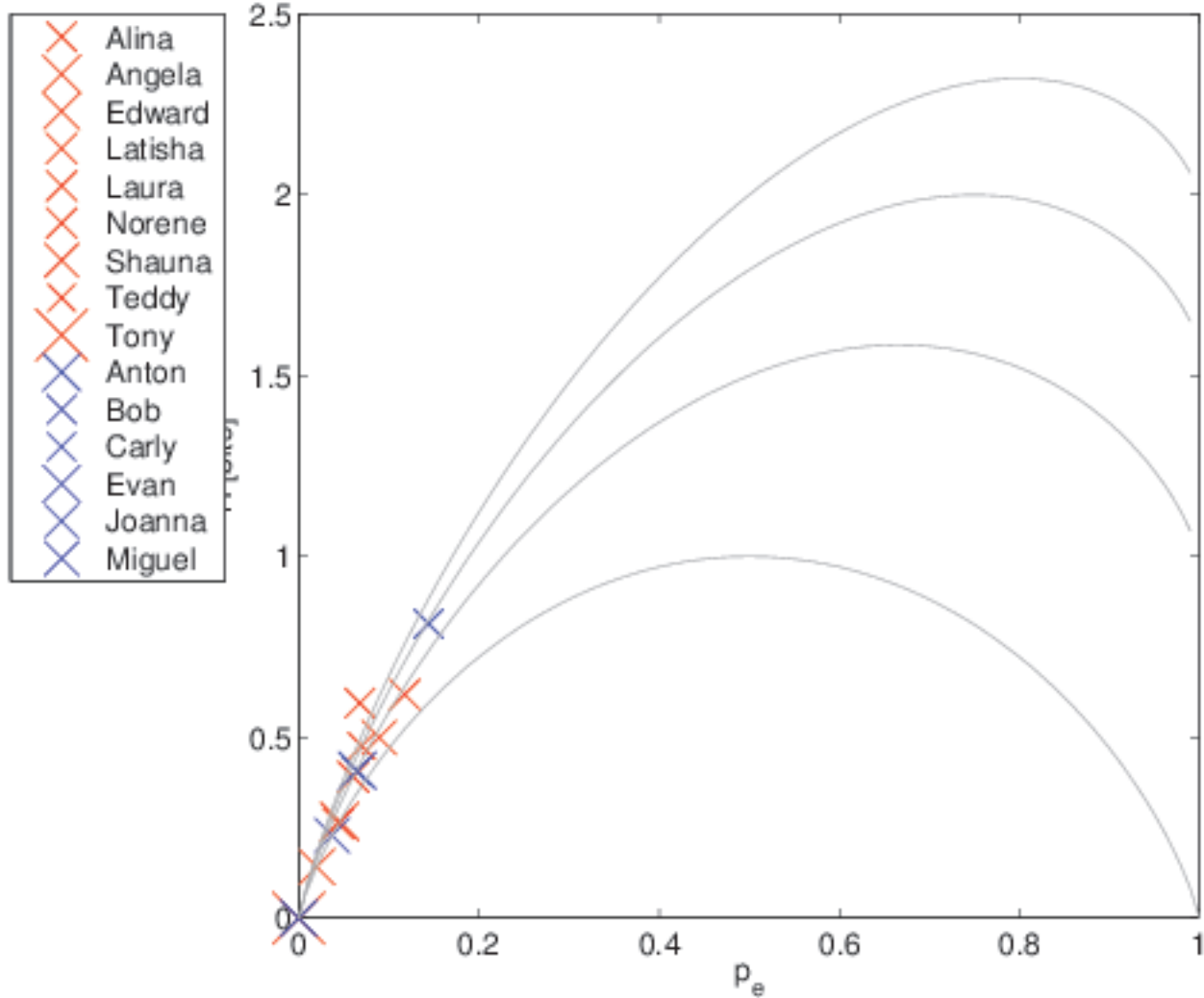
H(p_e) for Letter (m) in Initial Position
