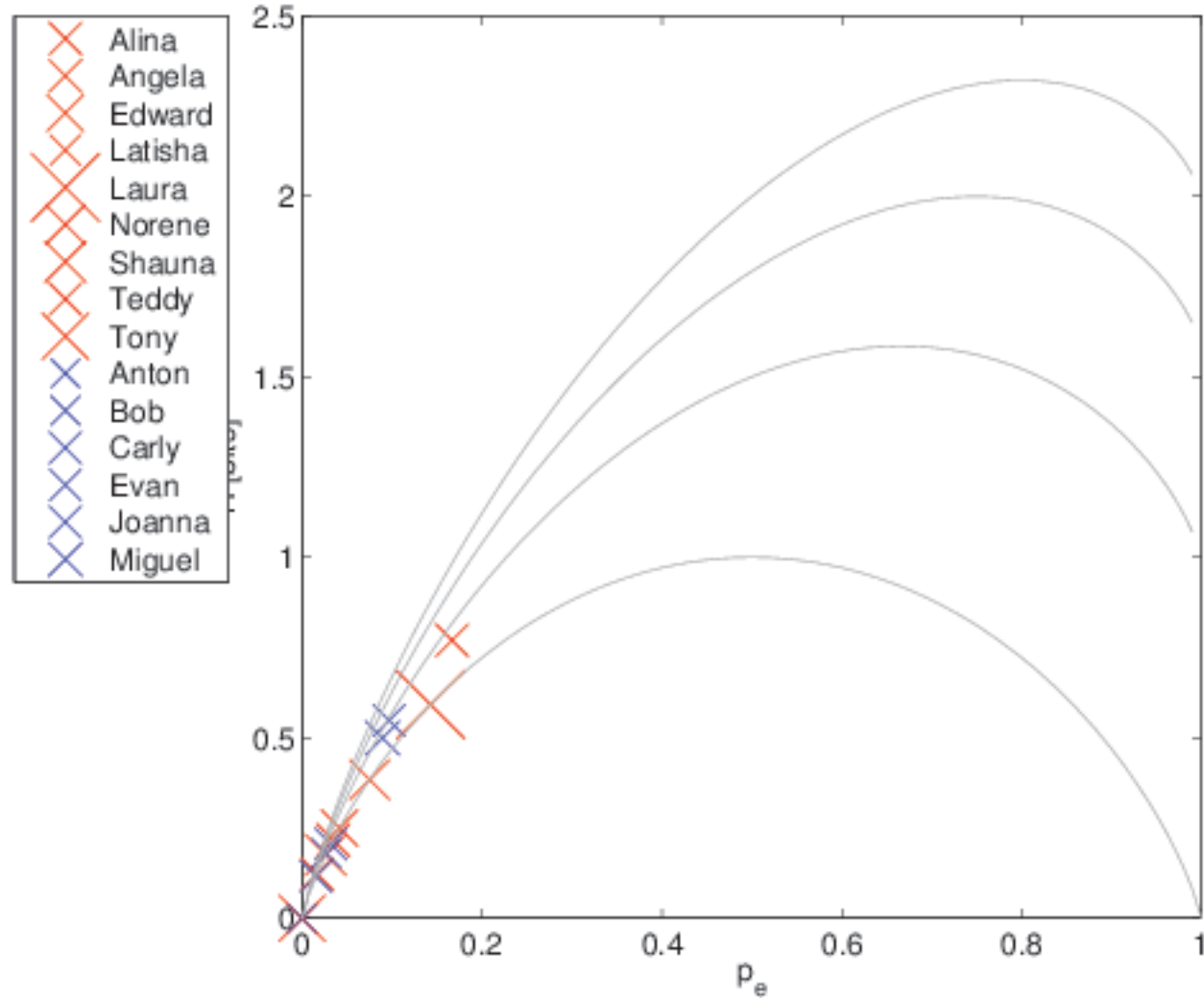
H(p_e) for Letter (n) in Initial Position
