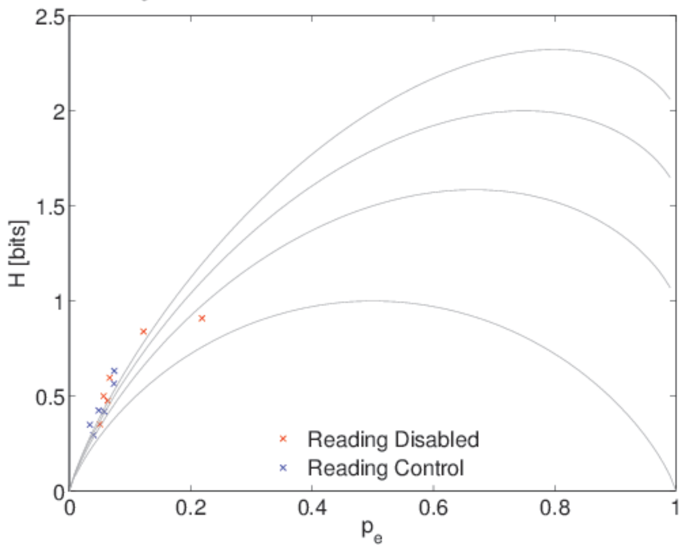
H(p_e) for Targets (nasalsLiquidsGlides) in Initial Position
