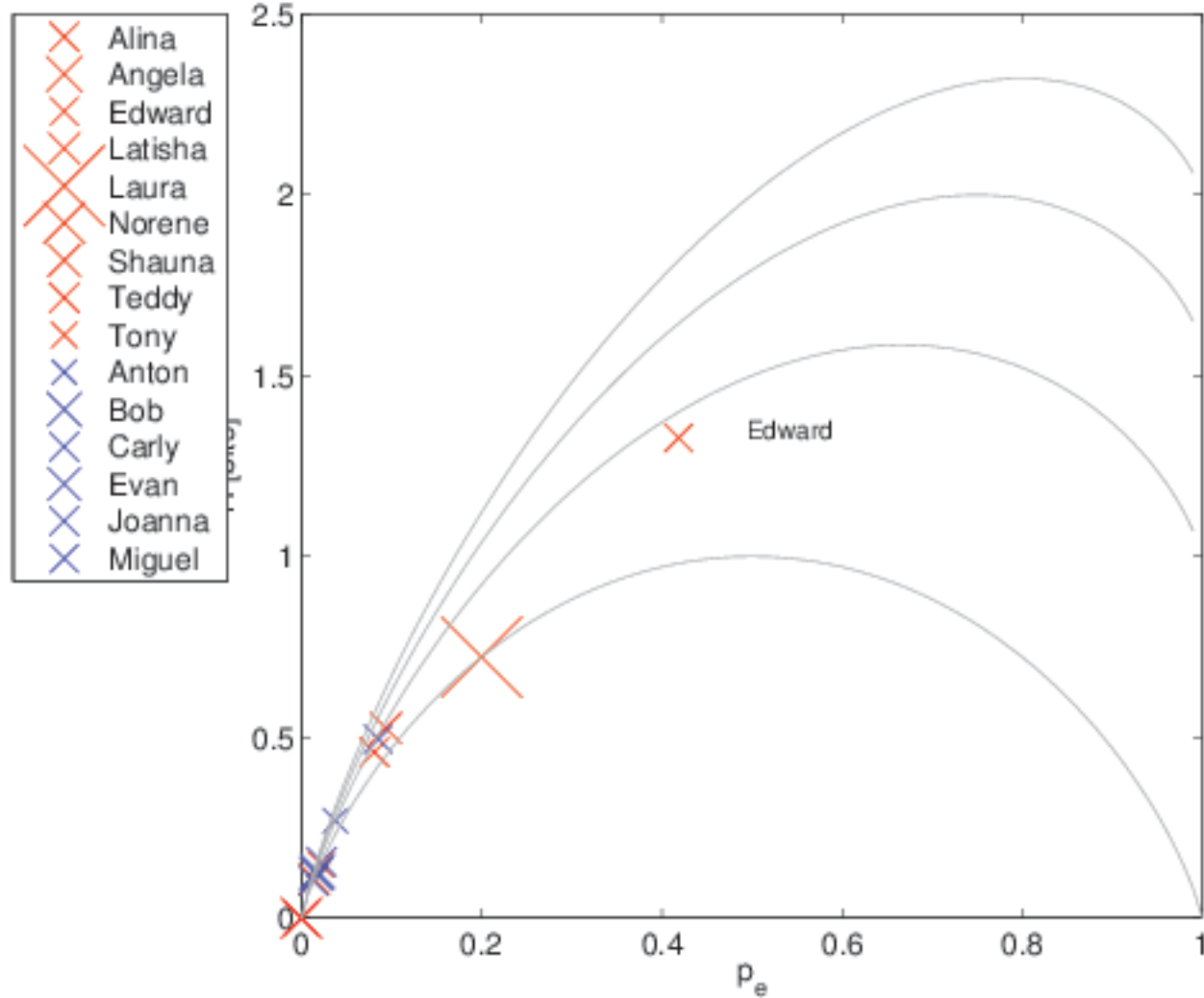
H(p_e) for Letter (s) in Initial Position
