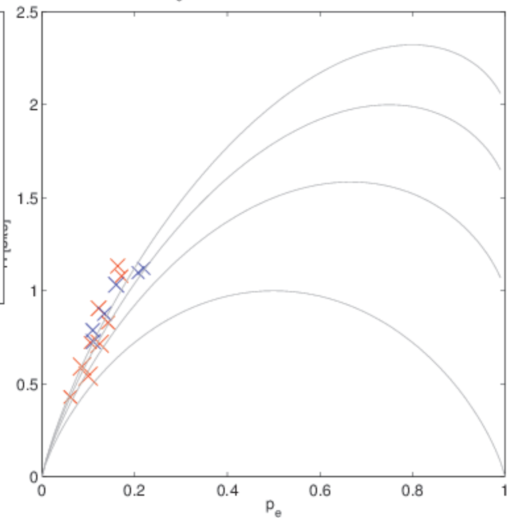
H(p_e) for Letter (u) in Initial Position
