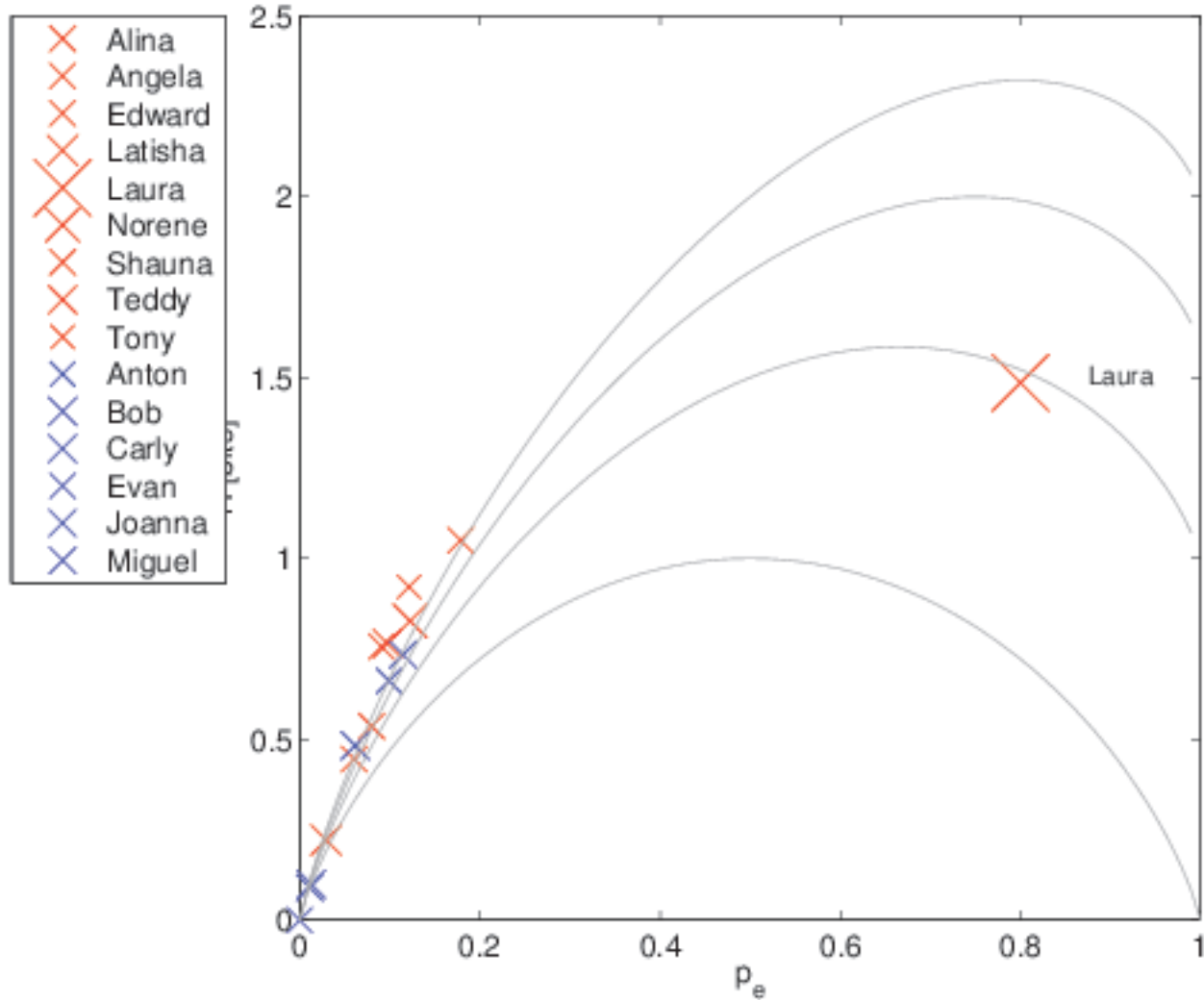
H(p_e) for Letter (Y) in Initial Position
