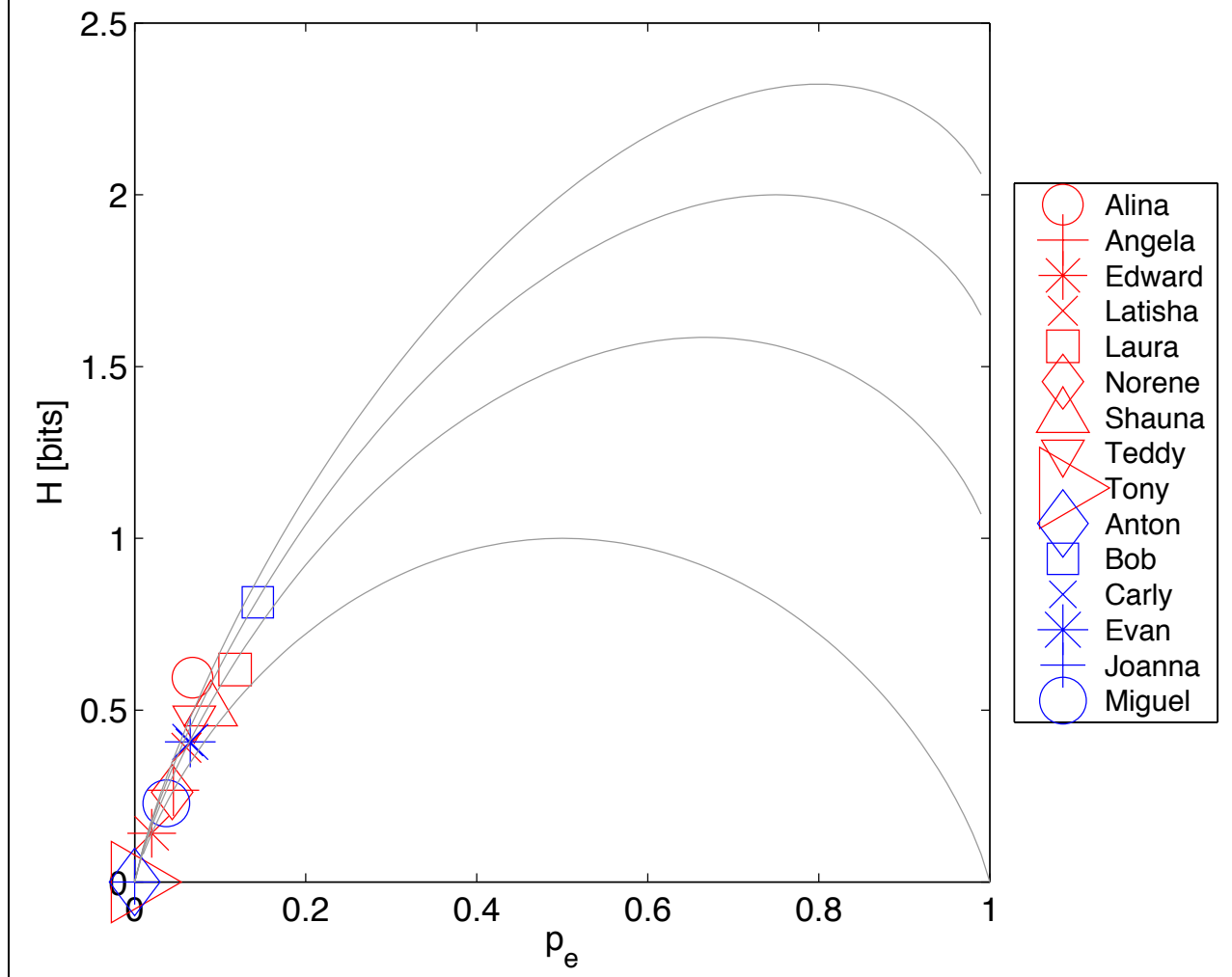
H(p_e) for Letter (m) in Initial Position
