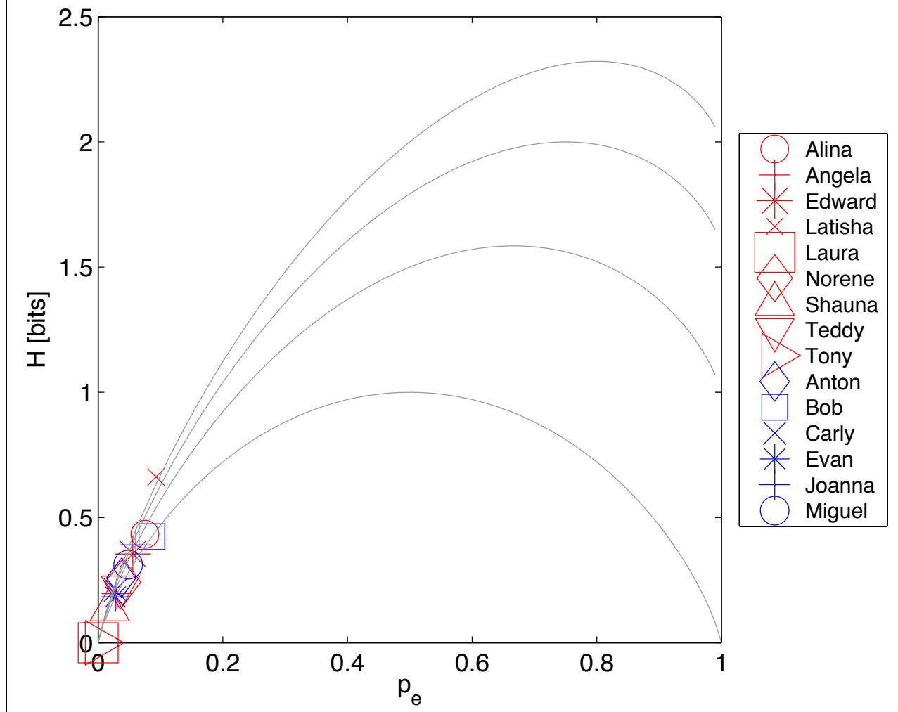
H(p_e) for Letter (t) in Initial Position
