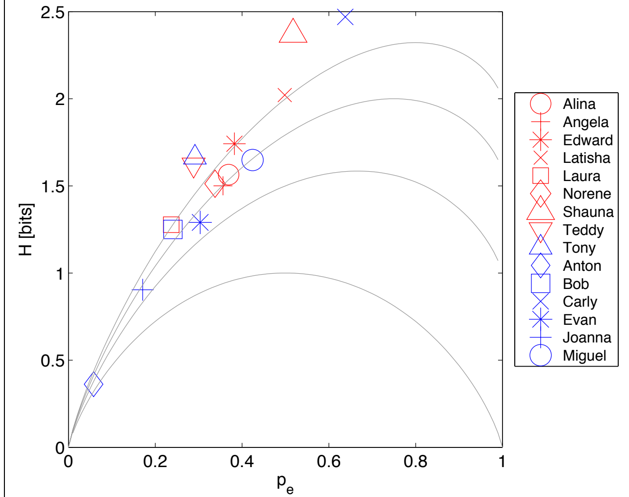
H(p_e) for Letter (T) in Final Position
