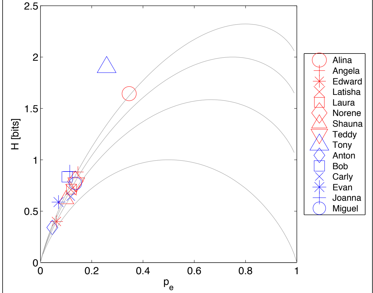
H(p_e) for Letter (p) in Final Position
