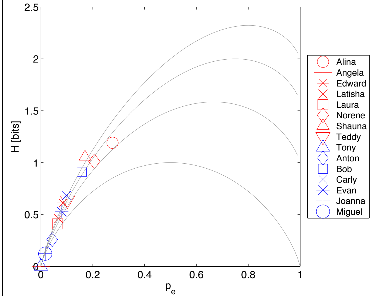
H(p_e) for Letter (S) in Final Position
