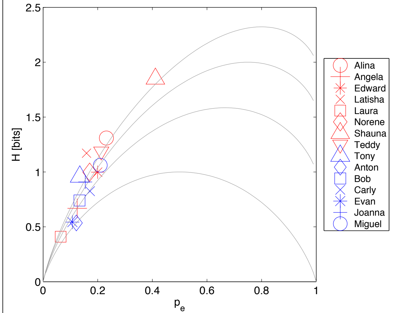
H(p_e) for Letter (m) in Final Position
