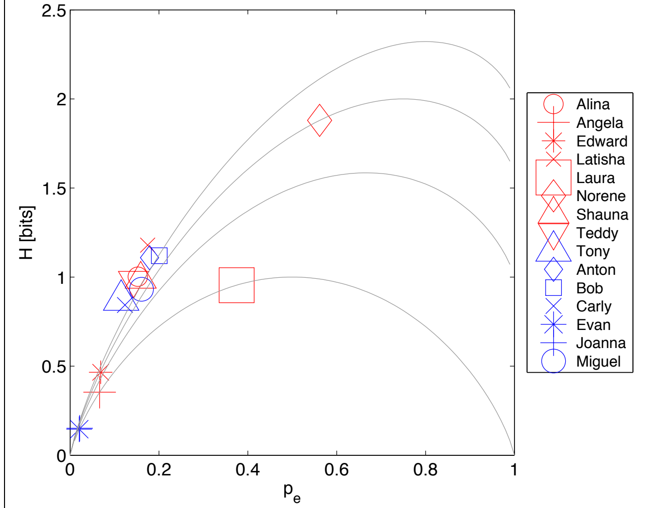
H( p_e ) for Letter (g) in Final Position
