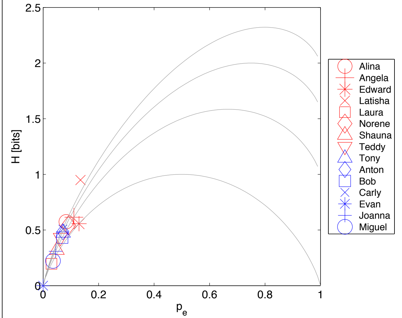
H(p_e) for Letter (C) in Final Position
