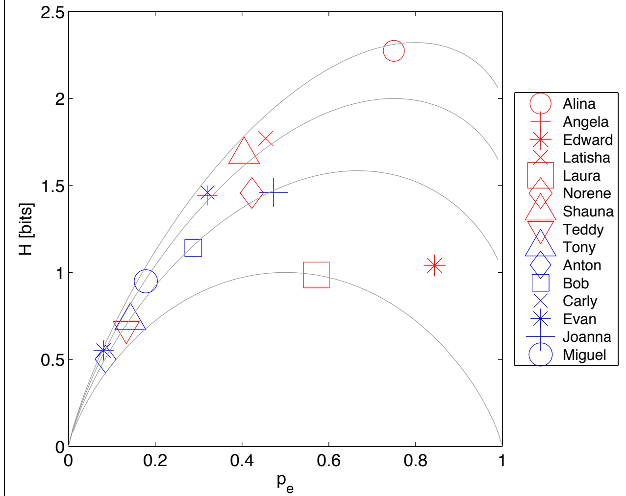
H(p e ) for Letter (Z) in Final Position
