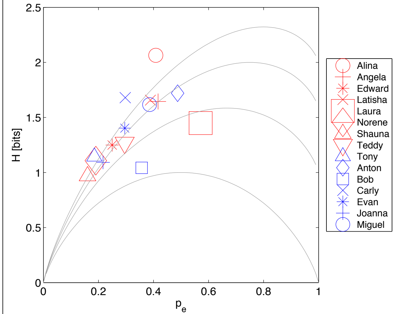
H(p_e) for Letter (G) in Final Position
