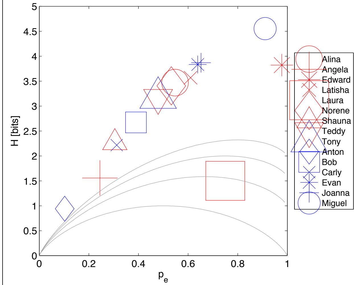
H(p_e) for Letter (r) in Final Position
