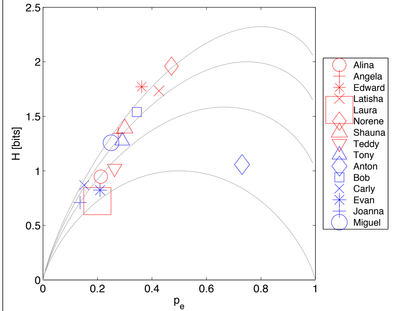
H(p_e) for Letter (f) in Final Position
