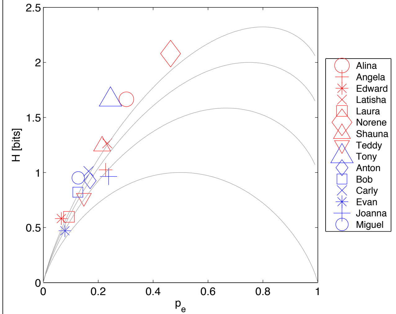
H(p_e) for Letter (b) in Final Position
