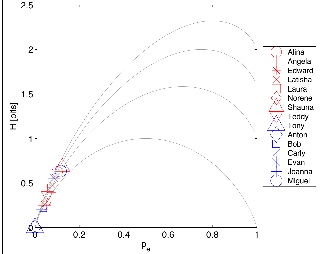
H(p_e) for Letter (k) in Final Position
