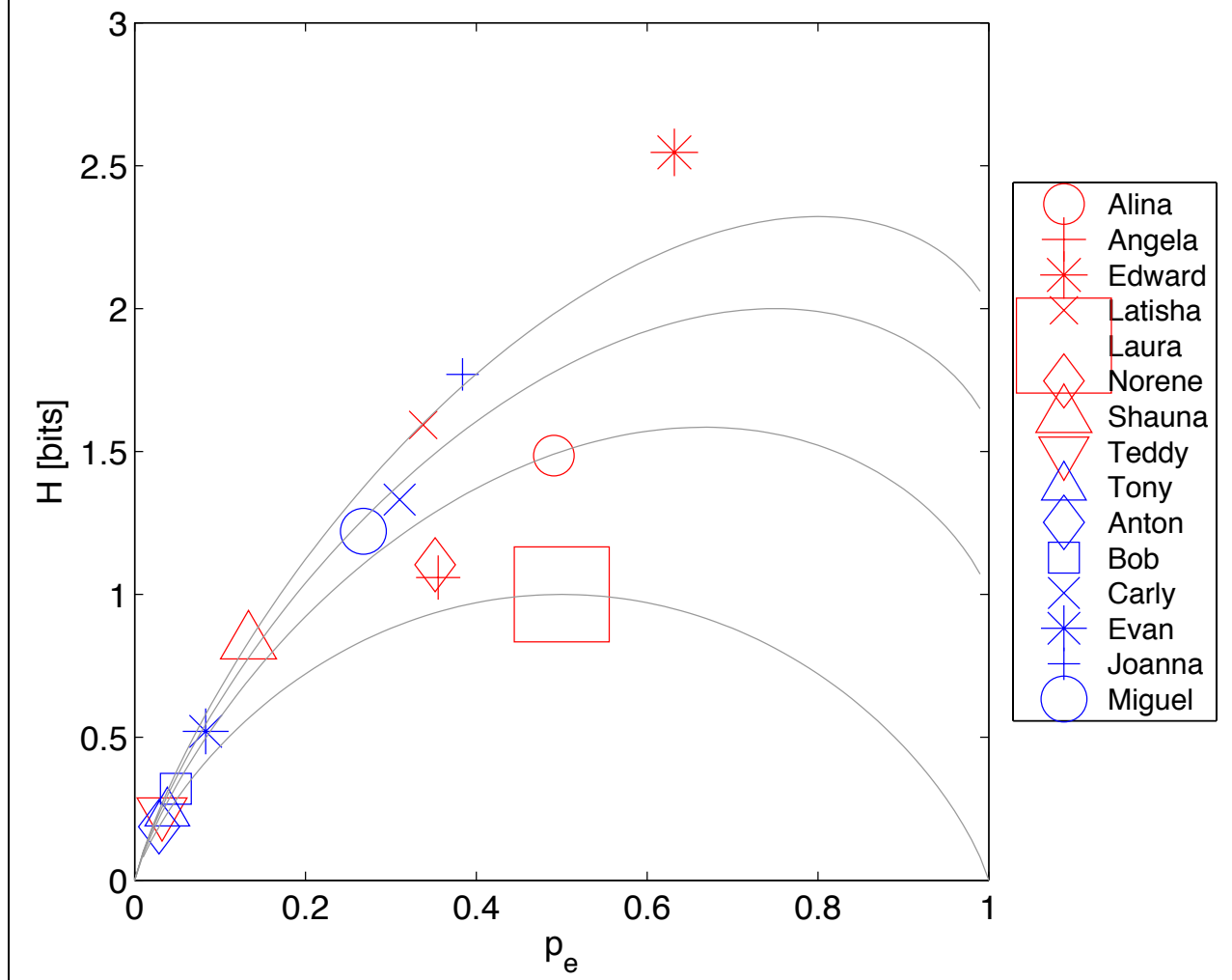
H(p_e) for Letter (z) in Final Position
