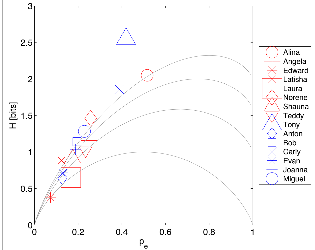
H(p_e) for Letter (n) in Final Position
