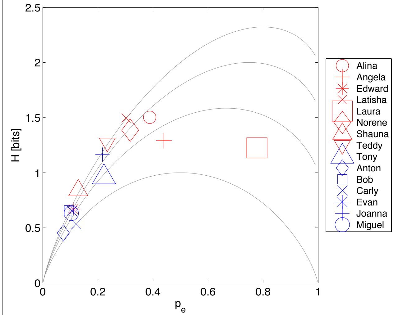
H(p_e) for Letter (J) in Final Position
