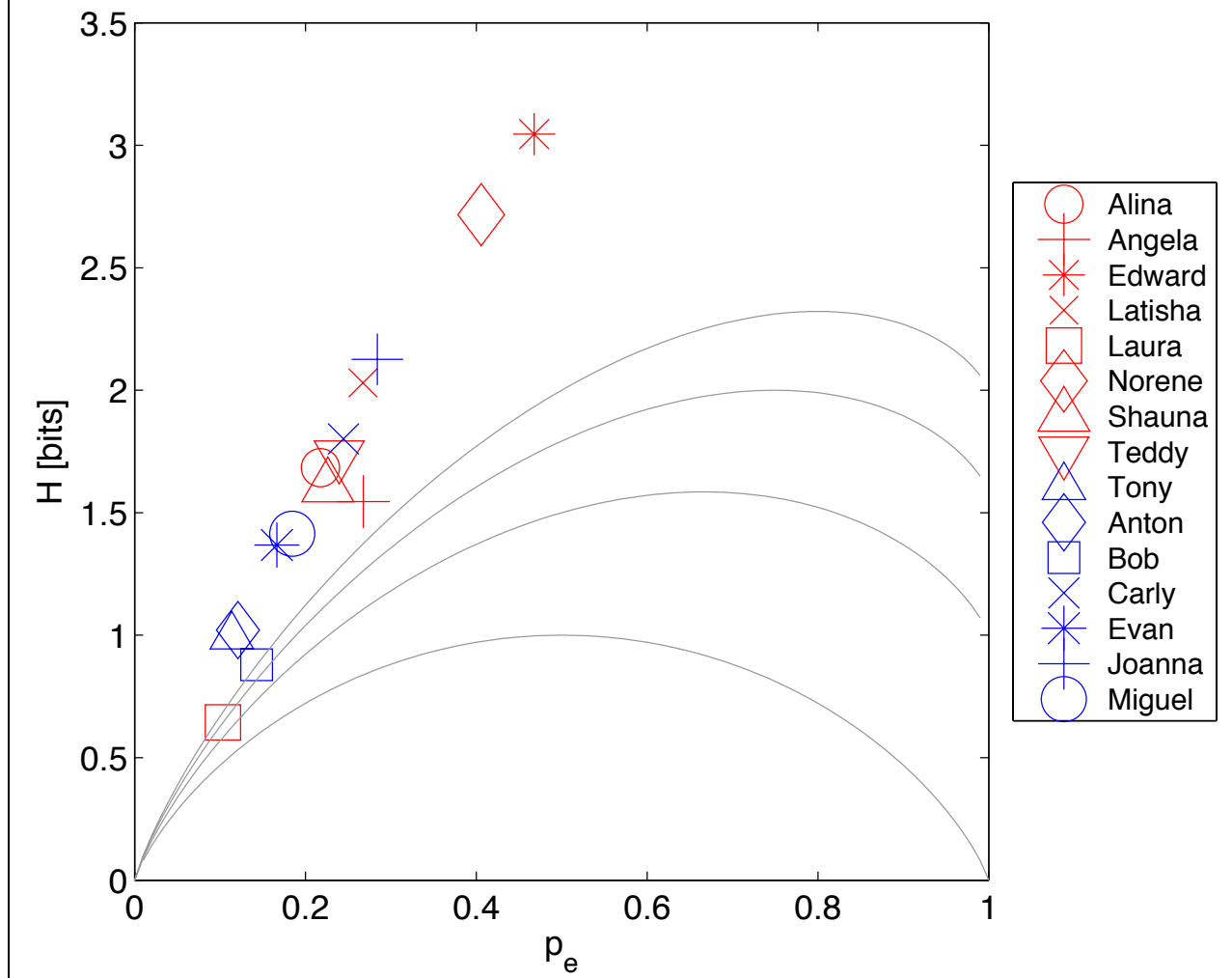
H(p_e) for Letter (L) in Final Position
