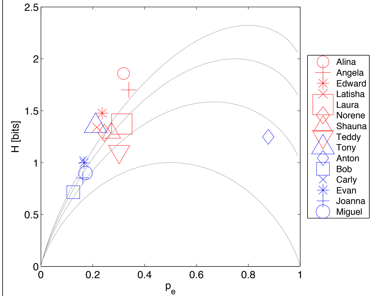
H(p e ) for Letter (v) in Final Position
