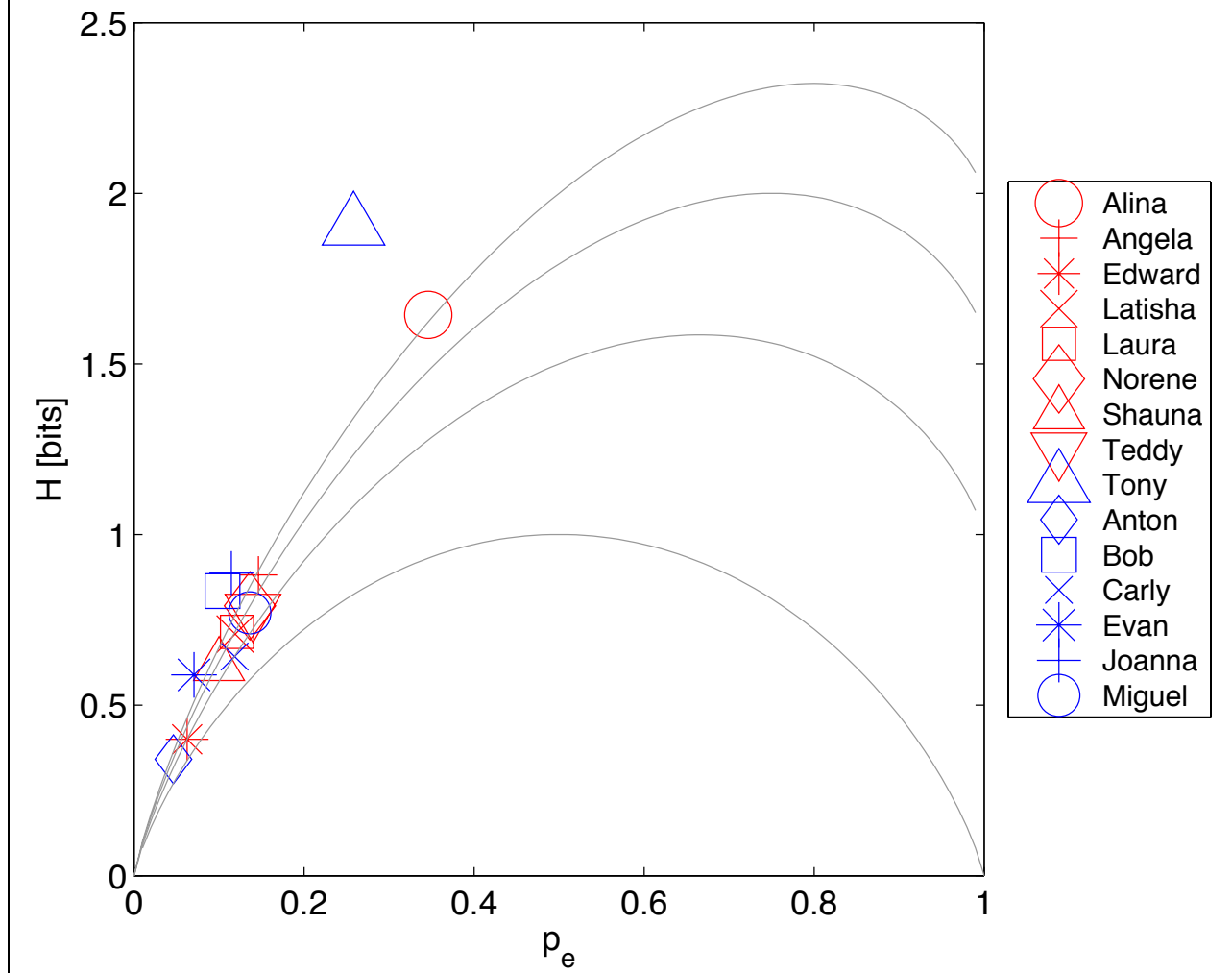
H(p_e) for Letter (p) in Final Position
