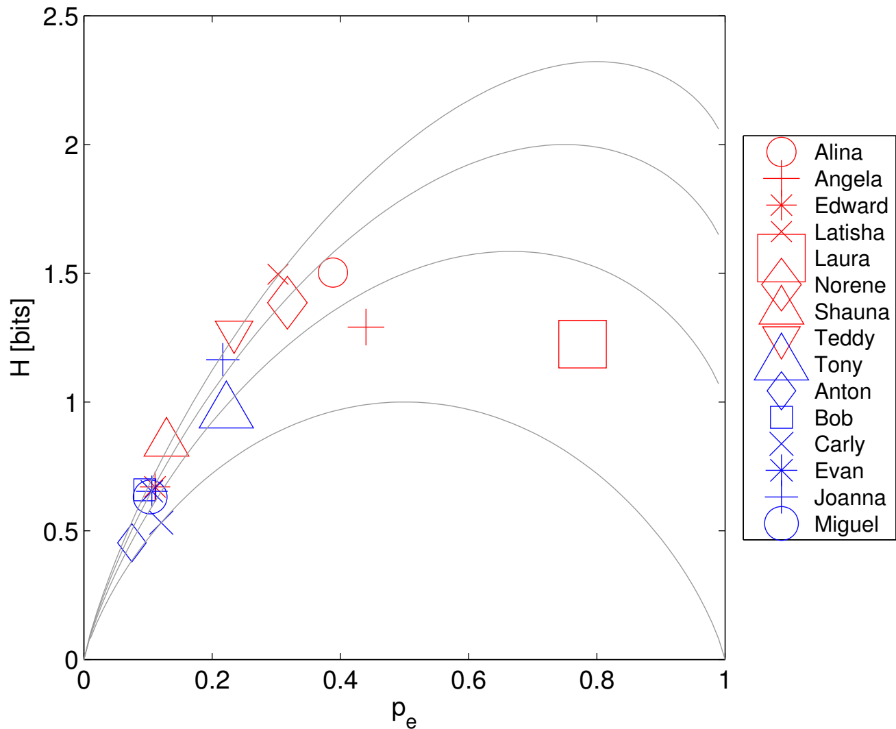
H(p_e) for Letter (J) in Final Position
