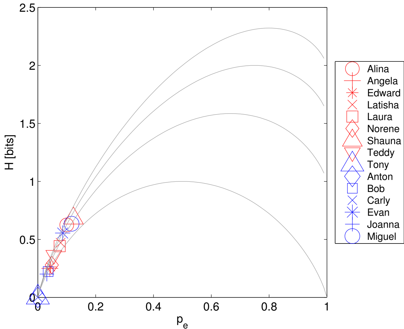
H(p_e) for Letter (k) in Final Position
