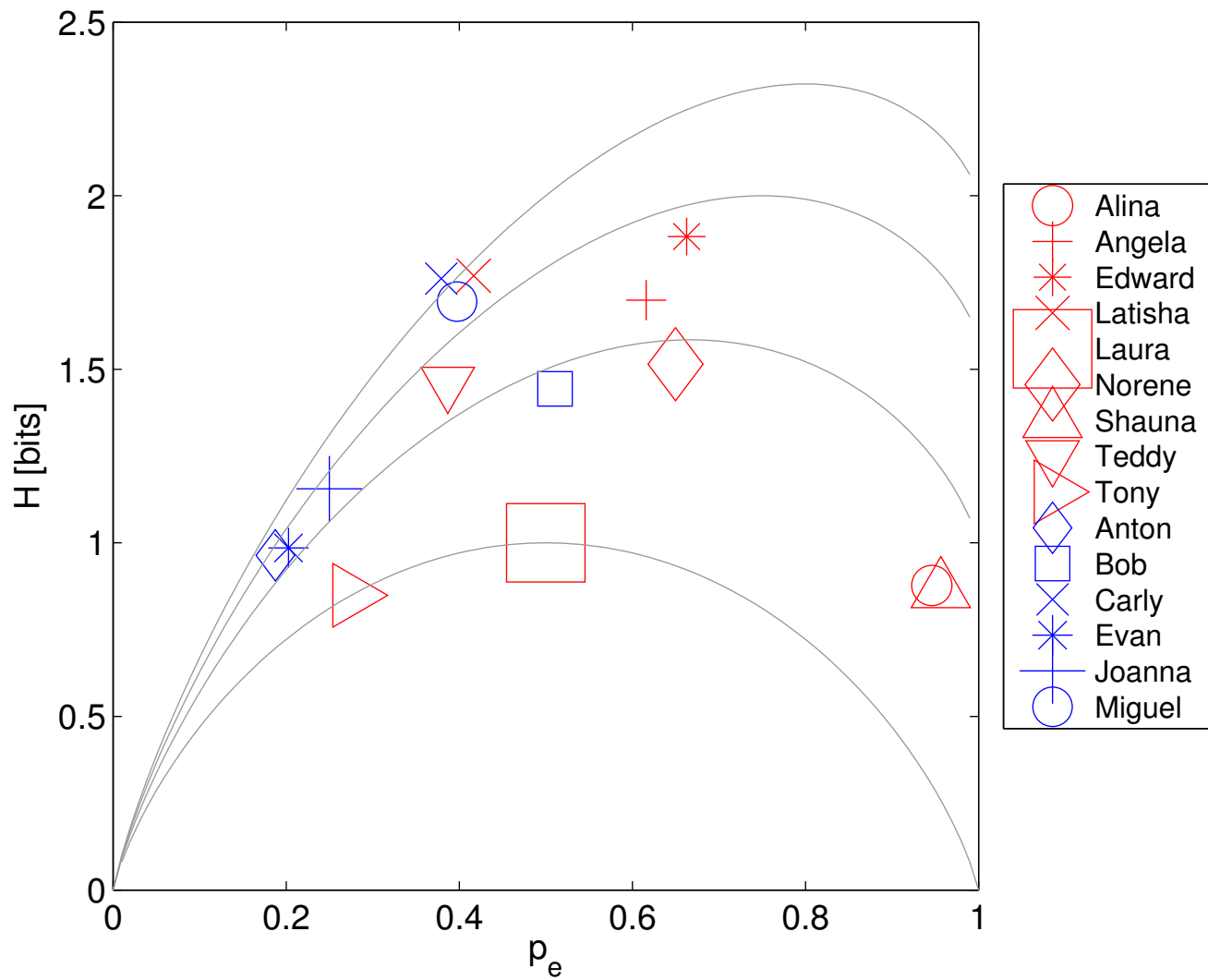
H(p_e) for Letter (Z) in Initial Position
