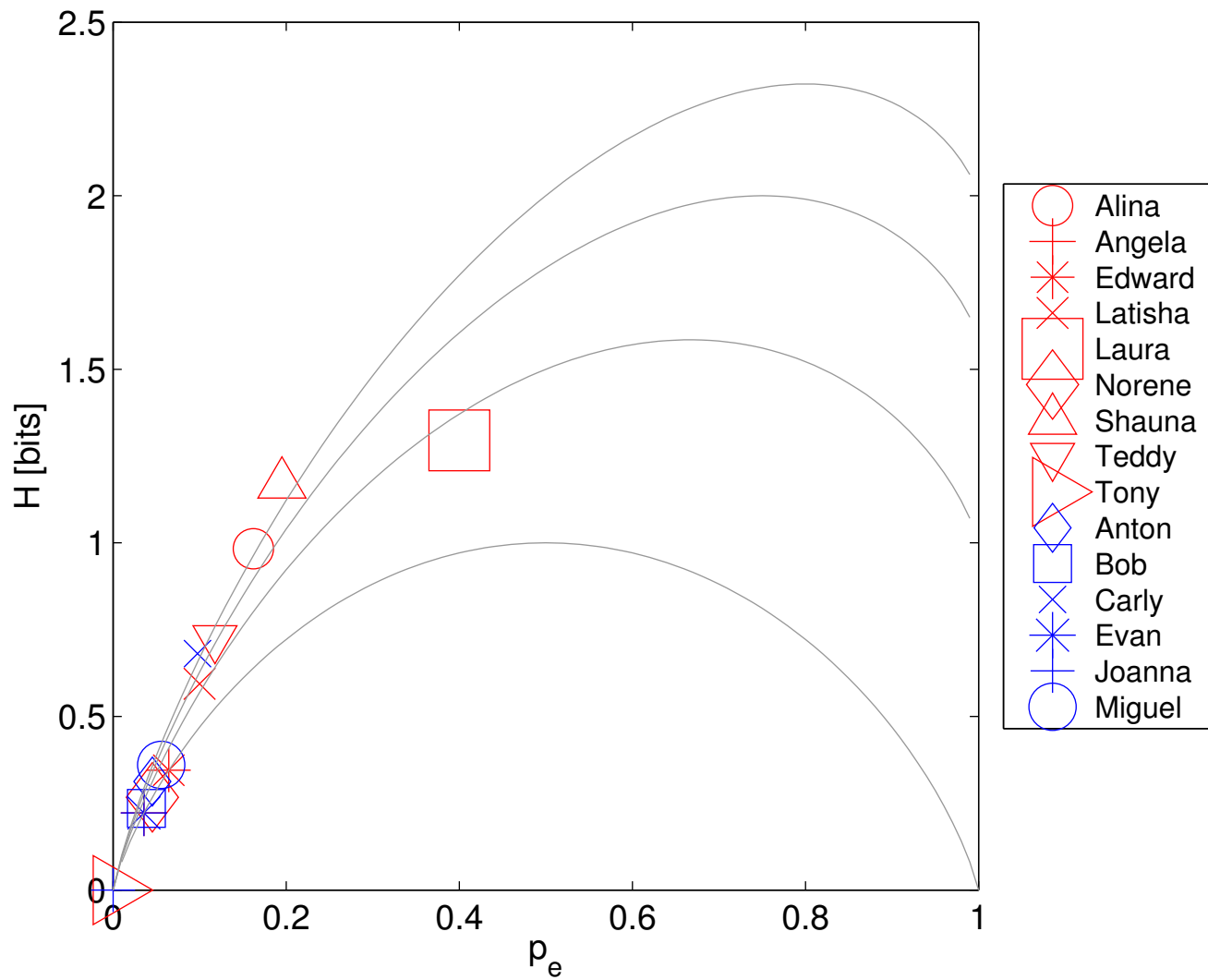
H(p_e) for Letter (g) in Initial Position
