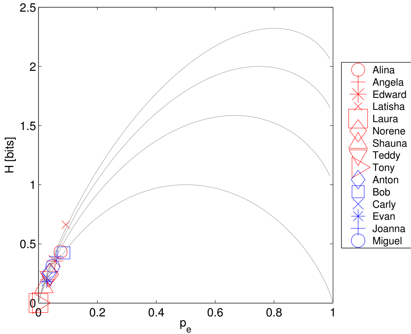
H(p_e) for Letter (t) in Initial Position
