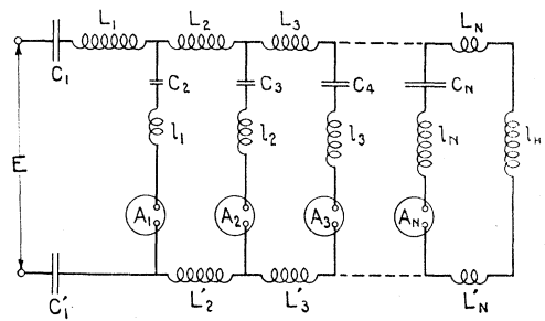
FIG. 7b. Electrical analogue of the cochlea.
