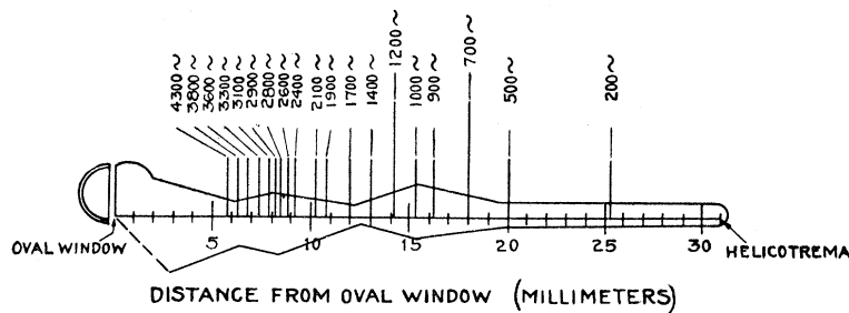
Fig. 12. Combinational tones.
