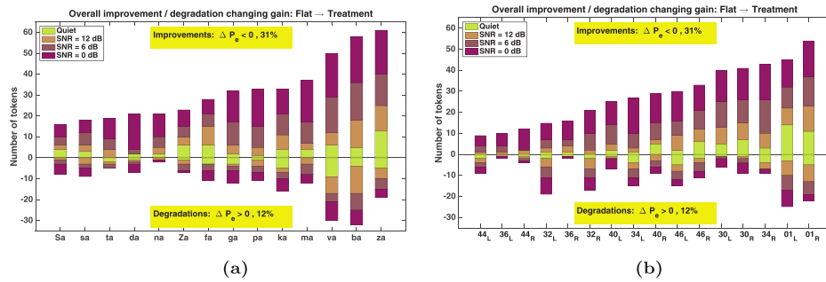
FIG. 4. (Color online) Overall number of token improvements ( \Delta P_e \leq 0 ) and degradations ( \Delta P_e > 0 ) due to the treatment. (a) Change in the number of errors as a function of the presented consonant + /a/ (included all available tokens for such consonant). Note the usage of symbol “S” to identify consonant /ʃ/, symbol “Z” to identify consonant /ʒ/, and symbol “a” to identify vowel /a/. (b) Change in the number of errors as a function of the individual ears. The positive direction indicates an improvement, while the negative direction indicates a degradation. The gray-scale code shows different SNRs (a darker shade represents higher noise). The highlighted percentage shows the net improvements (31%) and degradations (12%) across all presentations.
