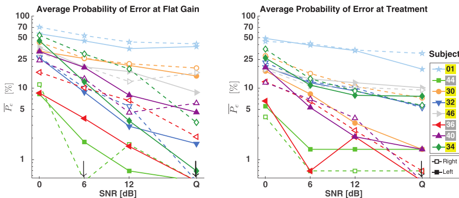
FIG. 5. (Color online) Average probability of error [ P_e(Ear, SNR) ] for all ears in log-percent (%) versus SNR [dB] for the flat (left) and treatment (right) gain experiments. Each line represents an ear [solid lines (closed symbols): left ear, dashed lines (open symbols): right ear]. Wherever P_e(Ear, SNR) is zero, the curves are truncated at the bottom of the plot (shown by ↓).
