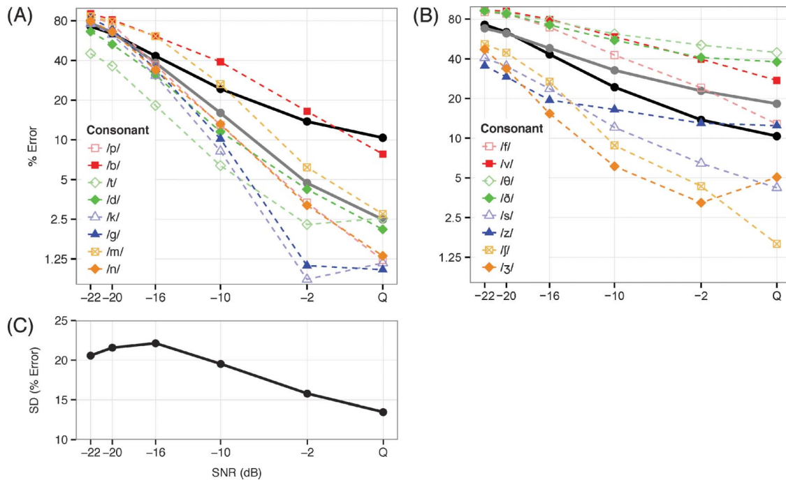
Figure 1. Mean consonant error ( e_c ) by SNR. The quiet (Q) condition is plotted at +5 dB SNR. The stops and nasals are shown in the left panel (A), and the fricatives are shown in the right panel (B). The solid black line is the grand mean across consonants ( e ), and the solid gray line shows the mean in each panel to visualize the differences between each subset of sounds. The lower panel (C) shows the SD of the mean error across all the consonants.
