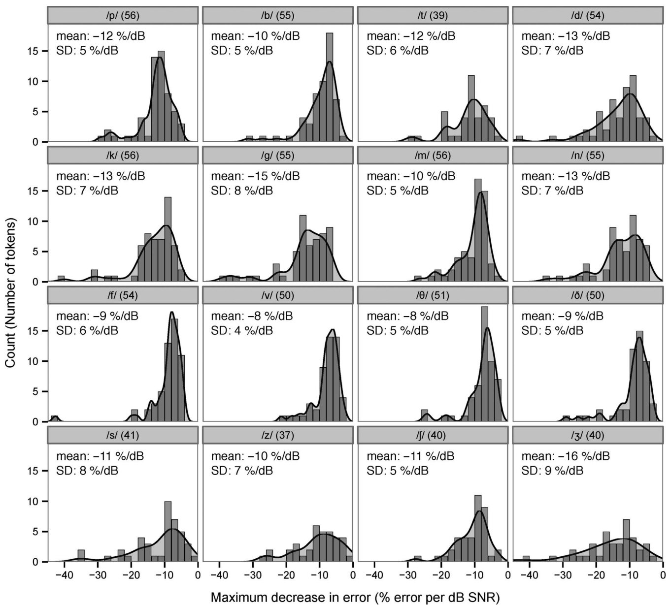
Figure 5. Histogram of the maximum slope (in magnitude) of the error function for each token as characterized by splines fits to e_r . The units are in %/dB. Many of the distributions peak at -10\%/dB , meaning that over a 10 dB range, the score would vary from no error to chance performance. The means and SDs of the distributions for each consonant are shown in the upper left corner of each panel.
