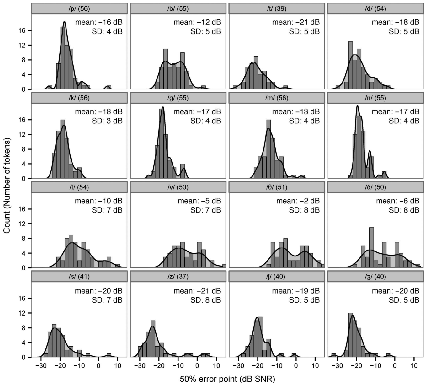
Figure 4. Histogram of SNR_{50} , defined by e_t = 0.5 , for each token ( t ), sorted by consonant ( c ). The SNR_{50} may be thought of as a detection threshold measure for the token. The mean and standard deviation (SD) are provided for each distribution, in the upper right corner of each panel. Some consonants have a very tight distribution with just a few sounds outside the 1 SD range. Others are nearly uniform about the mean. The further to the right on the mean, the less robust the token. Not surprisingly, high error sounds (mostly / \theta , \delta /) have a significant number of thresholds above 0 dB SNR. Note that one /s/ token is not plotted because its SNR_{50} is very low (less than -35 dB SNR).
