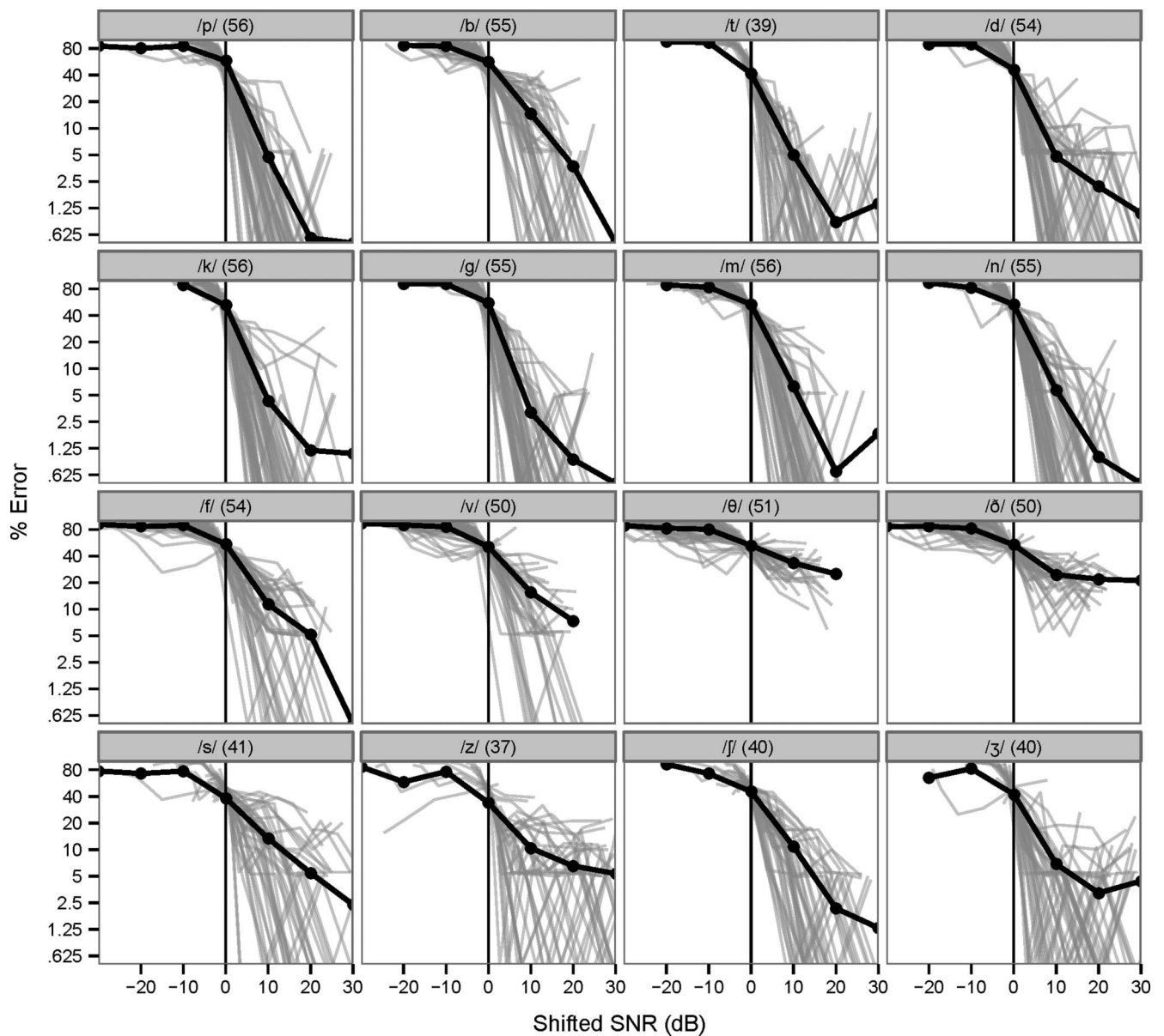
Figure 3. Percent log-error by SNR for each token (lines) sorted by consonant (panels). Each response was shifted along the SNR axis to the SNR_{50} for that token (i.e., e_t(SNR - SNR_{50}) for each token; Eq. 4). Above the SNR_{50} , e_t abruptly drops to zero, and below the SNR_{50} , it rises to chance. Thus, the differences in SNR_{50} across individual tokens account for a major source of the variance in e_t . Most of the natural variance has been removed in the shifted curves by simply accounting for this token-dependent parameter. The numbers after each consonant label indicate the number of tokens shown for that consonant (the maximum is 56).
