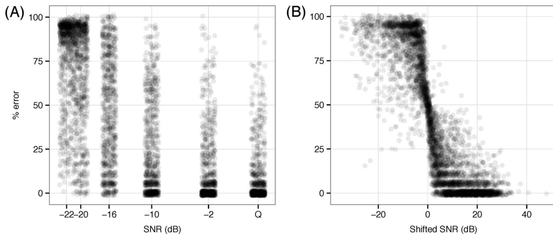
Figure 2. Panel A: Percent error for each token, as a function of SNR ( e_t(SNR) ). Panel B: Percent error shifted by the token's SNR_{50} , e_t(SNR - SNR_{50}) . In the left panel (A), the considerable variability among the error rates for each token is evident. After shifting by the token's SNR_{50} (Panel B), this variability is greatly reduced, revealing the step-function (e.g., binary) nature of the error. Data points are jittered slightly to prevent overplotting.
