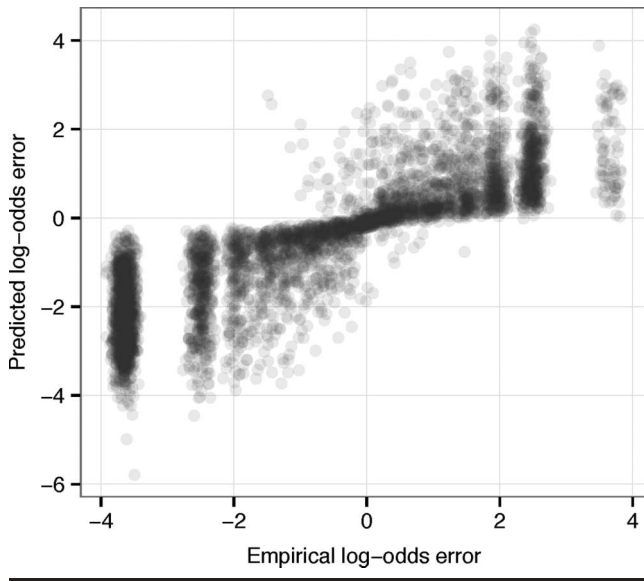
Figure 6. Scatter plot showing proportion of listeners' errors and predicted model responses for the regression model that accounted for differences in token-level error thresholds ( SNR_{50} ). Data points are jittered slightly to prevent overplotting.
