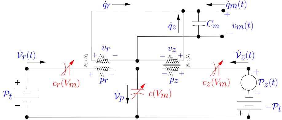
Figure 2. Final circuit diagram with turgor pressure as the source. Since the net volume at acoustic frequencies must be zero, \dot{V}_z = \dot{V}_r , and \dot{V}_p = 2\dot{V}_z .
