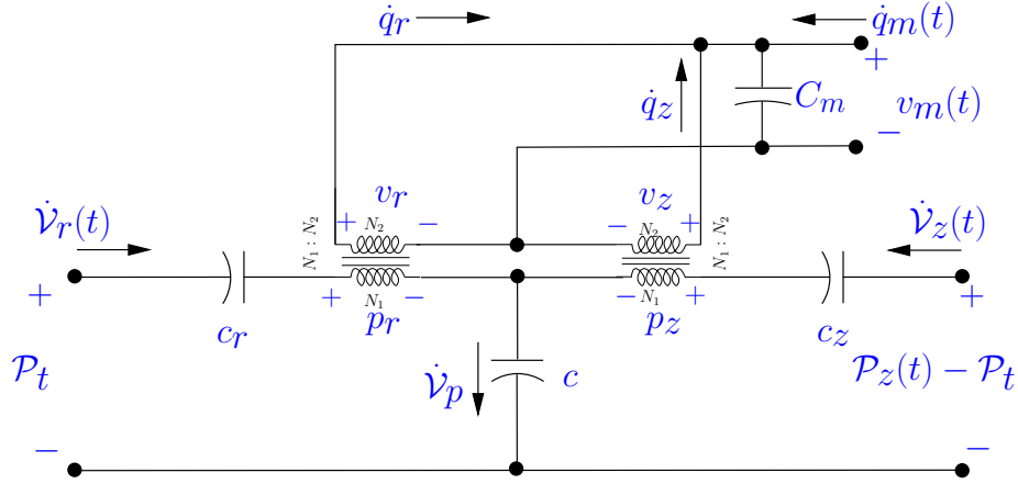
Figure 1. Circuit diagram corresponding to (8).
