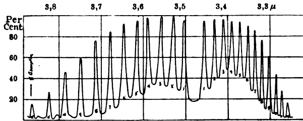
FIG. 102.—Rotation vibration spectrum of HCl, photographed by Innes by means of a reflexion grating of great dispersive power. The absorption per cent is plotted as the ordinate, and an angle of deflexion is plotted as the abscissa; the scale added above gives the corresponding wave-lengths in terms of \mu . The middle of the band (see the gap in the row of teeth) corresponds to \lambda = 3.46\mu .
