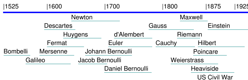
Figure 1: Time line showing some important mathematicians who lived between the 16-20 century.
