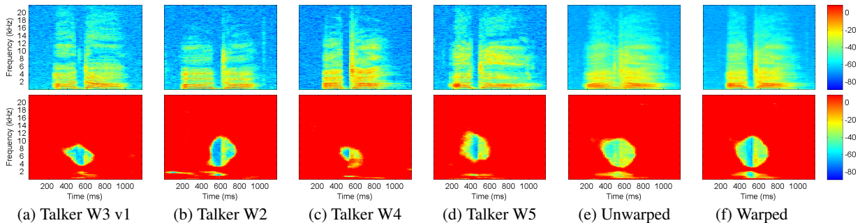
Figure 2: Spectrograms (top row) and time-frequency importance functions masking the spectrograms (bottom row) for four versions of the word ada spoken by different talkers (a)–(d) , and the pooled spectrogram and TFIF unwarped (e) and warped (f) to match W4.
