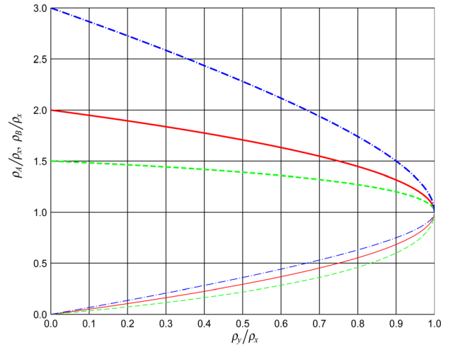
FIG. 3. (Color online) Mass densities of the equivalent two isotropic layers determined by those of the anisotropic layer, at three different thickness ratios: r = 0.5, 1, 2 . Solid curves: r = 1 . Dashed curves: r = 0.5 . Dot-dashed curves: r = 2 . Thicker curves: \rho_A ; thinner curves: \rho_B .
