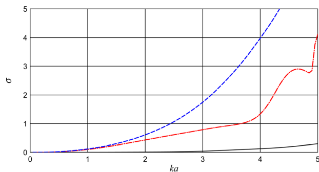
FIG. 4. (Color online) Normalized total scattering cross section \sigma of a rigid cylinder cloaked by cloaks comprising of 5 isotropic layer pairs. Each pair is impedance-matched. Solid curve: anisotropic cloak. Dot-dashed curve: proper placement—placing heavier layer in each pair closer to the object. Dashed curve: improper placement—placing softer layer in each pair closer to the object.
