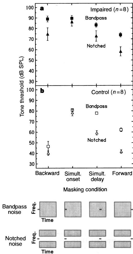
Figure 2 Average tone level required by eight language-impaired (a) and eight control (b) children to just detect a brief tone presented before, during or after a bandpass (squares, replotted from Fig. 1b) or notched (triangles) noise. Error bars indicate plus and minus one standard error of the mean across subjects. The stimuli are represented schematically along the bottom.
