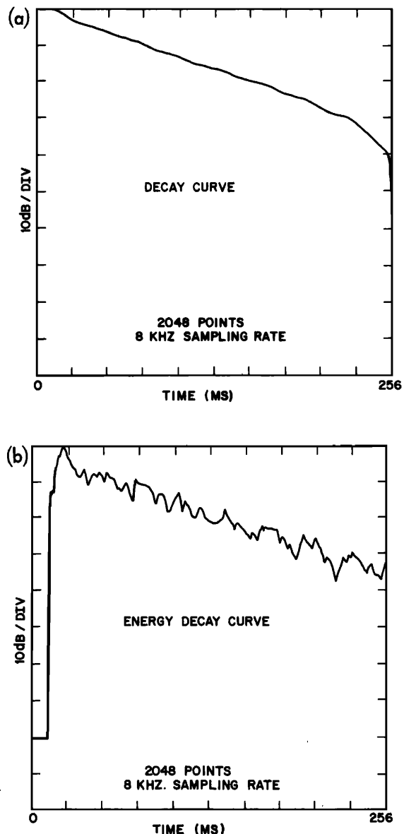
FIG. 3. (a) Energy decay curve for the impulse response of Fig. 2 using the Schroeder integration method. 22 (b) Impulse energy decay curve for a simulated level recorder.
