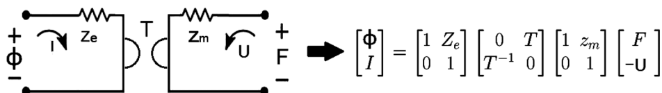
FIG. 2. A schematic representation of a two-port ABCD electro-mechanic system using Hunt parameters Z_e(s) , z_m(s) , and T(s) : electrical impedance, mechanical impedances, and transduction coefficient (Hunt, 1954; Kim and Allen, 2013). Also \Phi(f) , I(f) , F(f) , and U(f) are the frequency domain voltage, current, force, and volume velocity, respectively. Notice how the ABCD matrix method “factors” the two-port model into 2 \times 2 matrices. This allows one to separate the modeling from the algebra. The flow is always defined into the port. Thus it is necessary to force a negative sign on the volume velocity.
